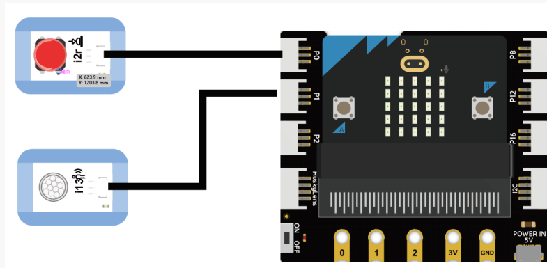
Connection diagram of micro: bit receiver:
