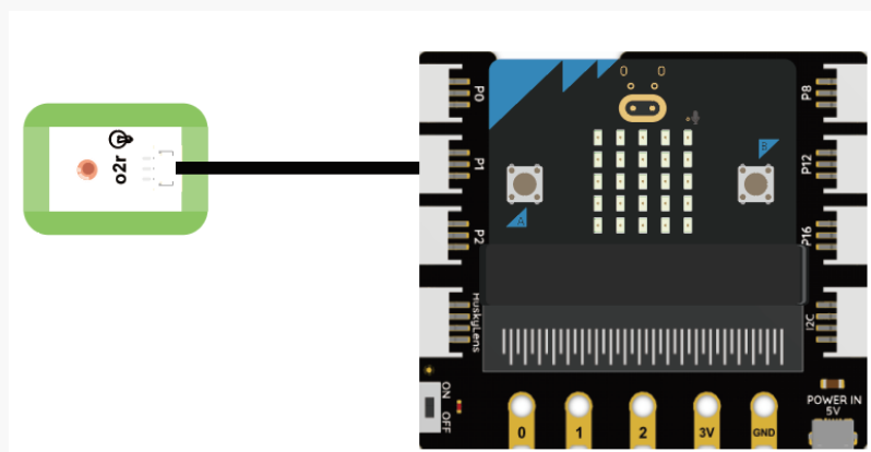
Connection diagram of micro: bit receiver:
