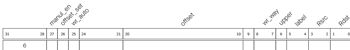
Figure 1.5-5. Instruction Type - ST
