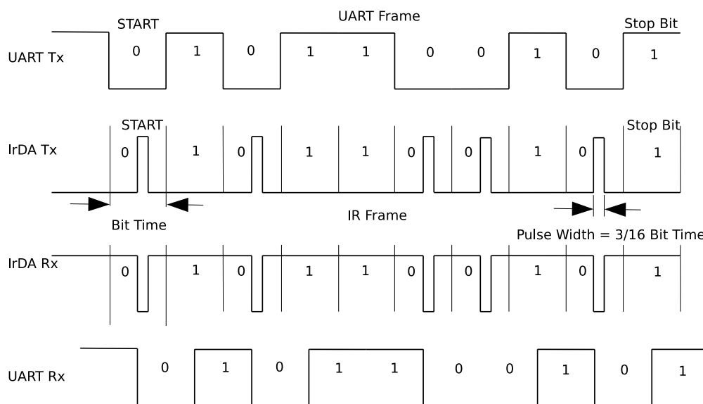
Figure 23.3-8. The Timing Diagram of Encoding and Decoding in SIR mode
