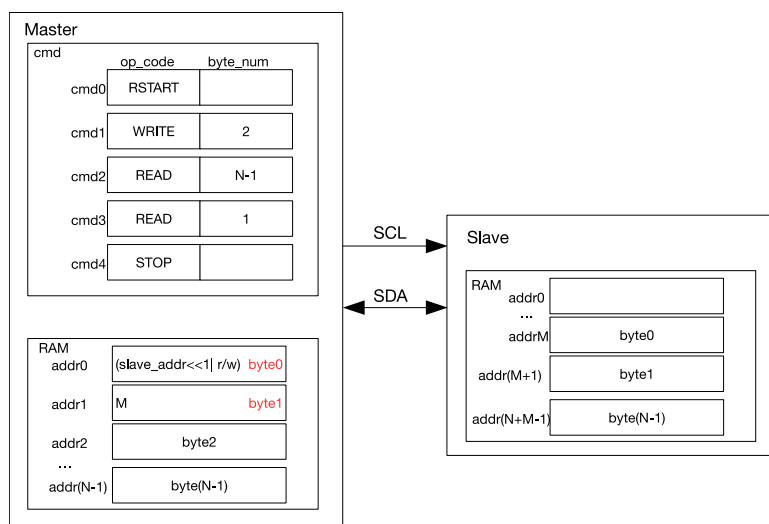
Figure 25.2-11. An I2C Master Reading N Bytes of Data from addrM of an I2C Slave with a 7-bit Address
