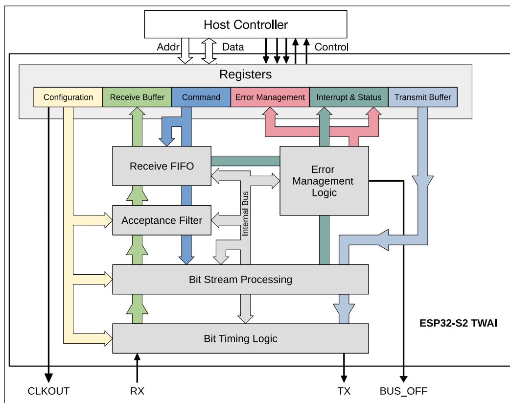
Figure 29.4-1. TWAI Overview Diagram
