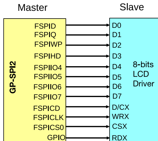
Figure 24.4-5. Connection of GP-SPI2 to 8-bit LCD Driver
