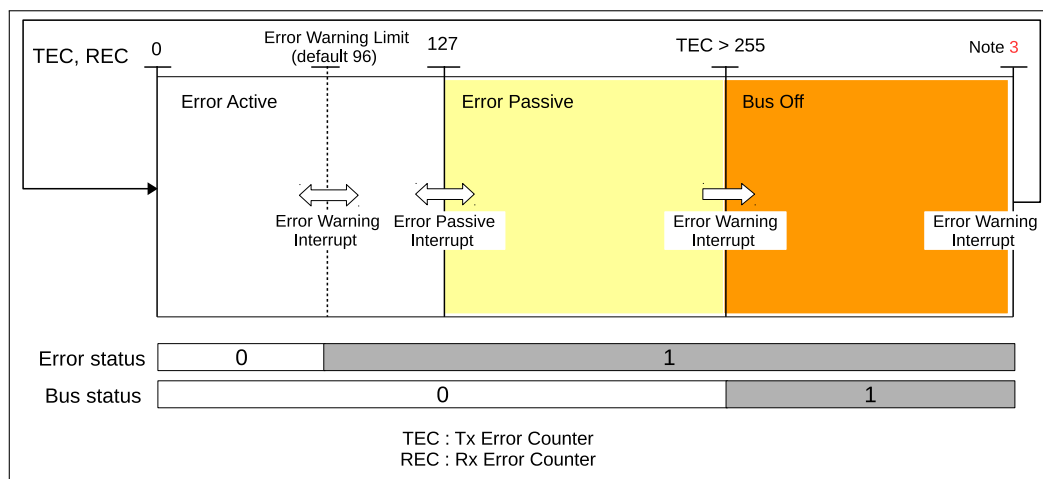
Figure 29.5-4. Error State Transition
