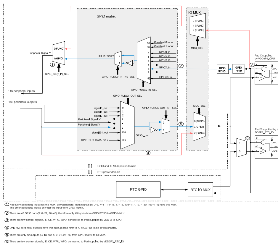
Figure 5.1-1. IO MUX, RTC IO MUX and GPIO Matrix Overview
