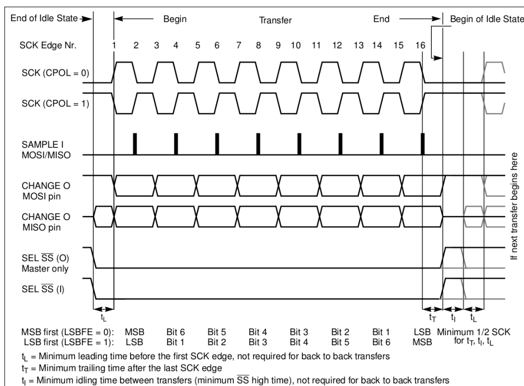
Figure 24.9-2. SPI CLK Mode 1 or 3
