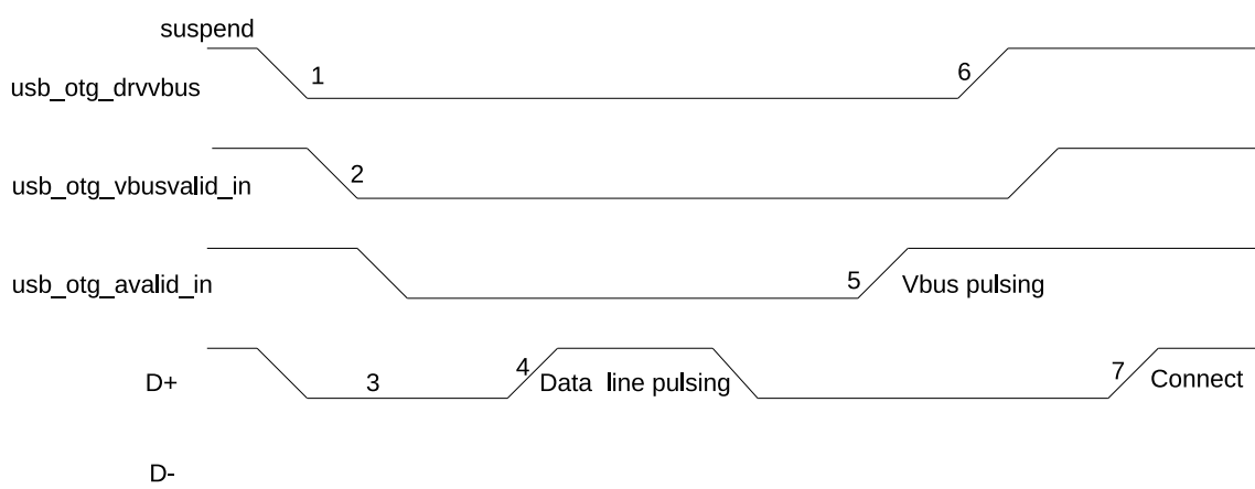
Figure 28.4-1. A-Device SRP
