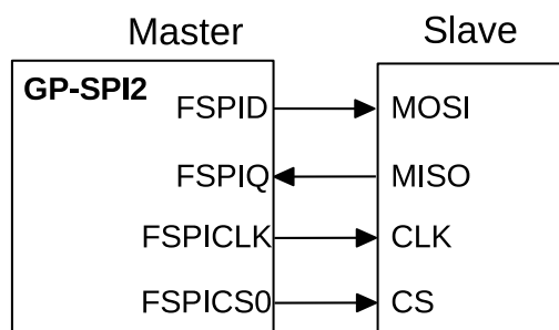
Figure 24.4-2. Full-Duplex Communication Between GP-SPI2 Master and a Slave
