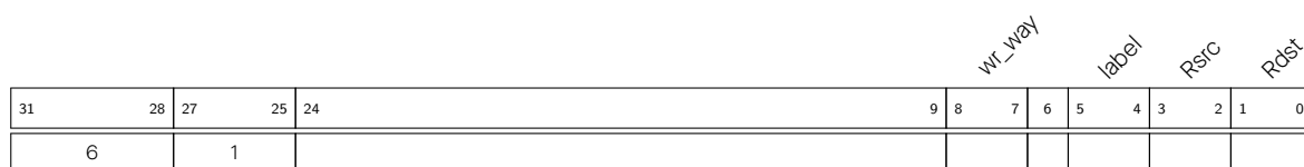
Figure 1.5-7. Instruction Type - Data Storage in Automatic Storage Mode (ST-AUTO-DATA)
