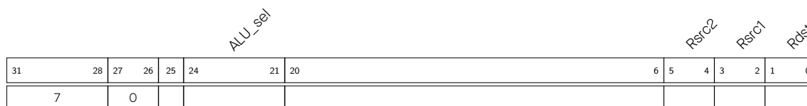
Figure 1.5-2. Instruction Type — ALU for Operations Among Registers
