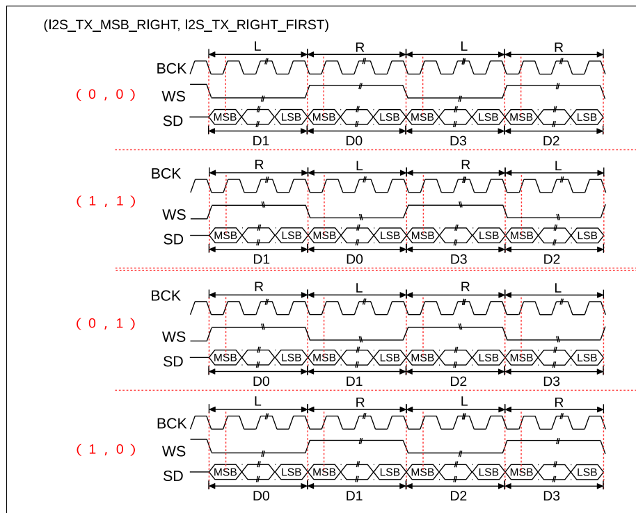
Figure 26.8-2. I2S Output Format When I2S_TX_CHAN_MOD[2:0] = 0 and I2S_TX_DMA_EQUAL = 0
