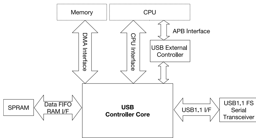
Figure 28.3-1. OTG_FS System Architecture
