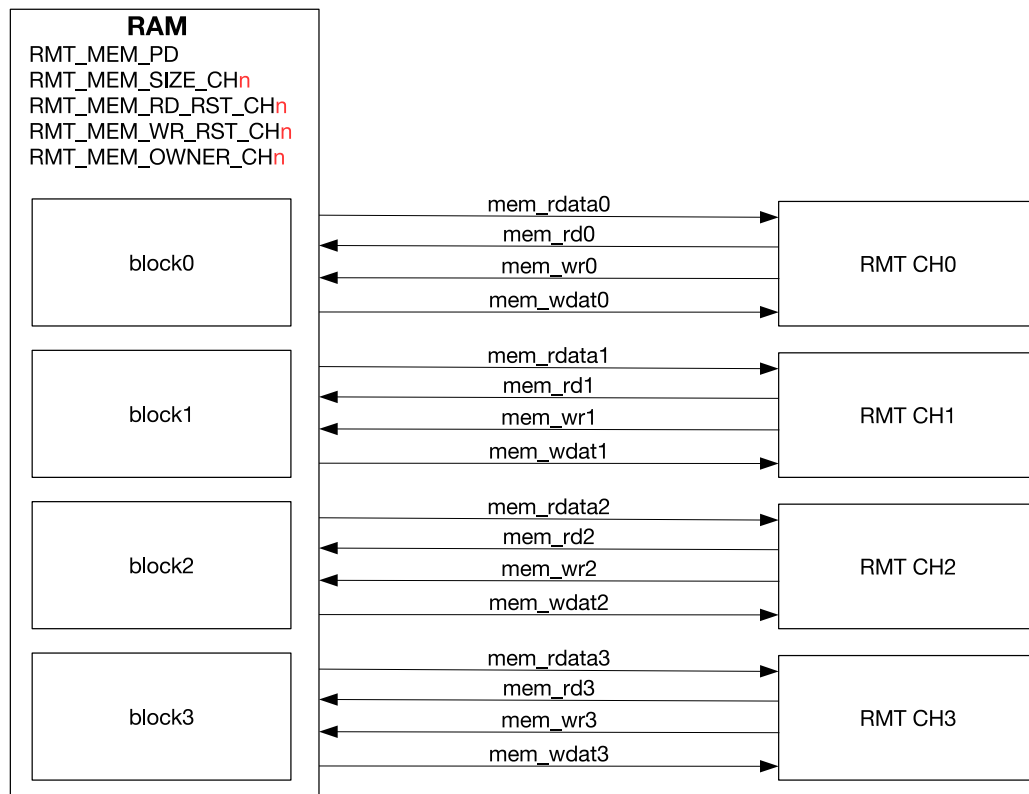
Figure 31.2-2. RMT Channels
