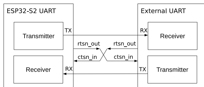
Figure 23.3-11. Connection between Hardware Flow Control Signals
