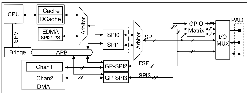
Figure 24.1-1. SPI Block Diagram
