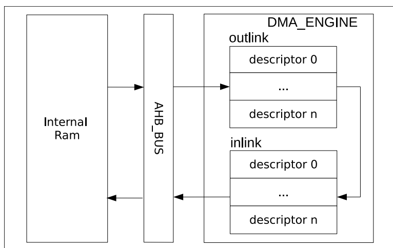
Figure 2.4-1. Copy DMA Engine Architecture
