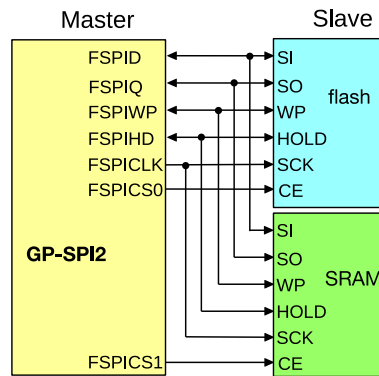
Figure 24.4-3. Connection of GP-SPI2 to Flash and External RAM in 4-bit Mode
