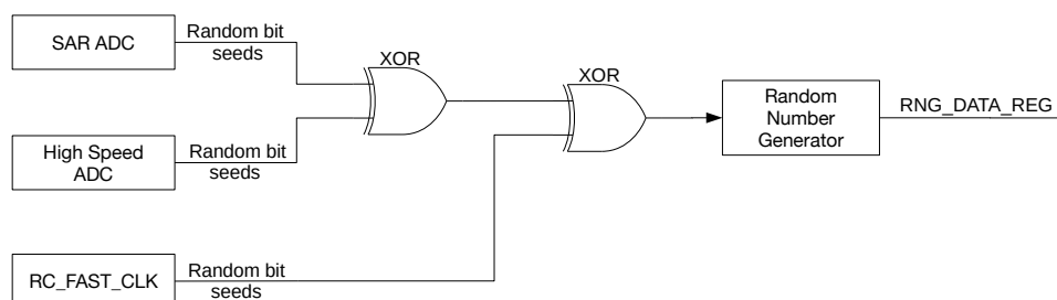
Figure 22.3-1. Noise Source
