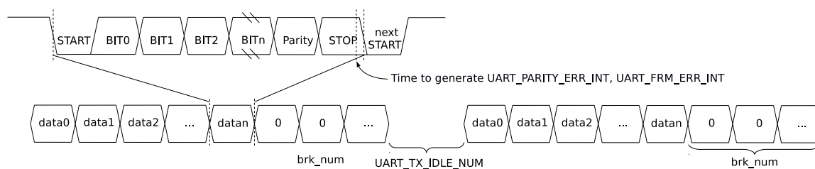
Figure 23.3-5. Structure of UART Data Frame
