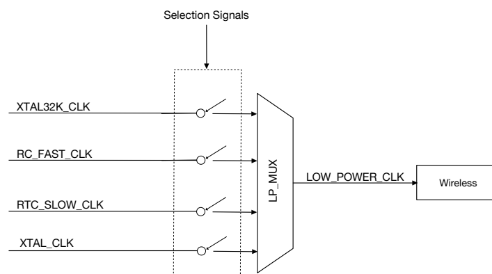
Figure 9.3-4. Low-Power Clocks for RTC Power Domains
