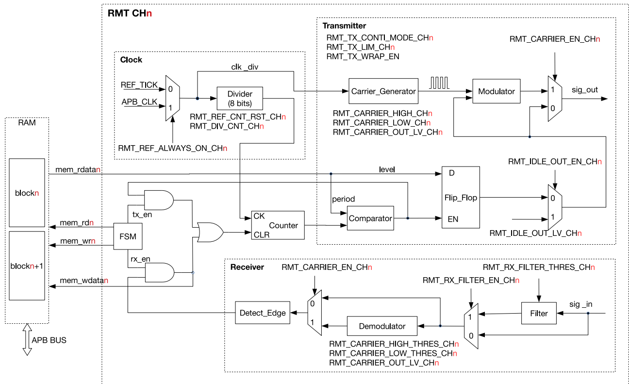
Figure 31.2-1. RMT Architecture
