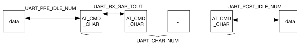
Figure 23.3-6. AT_CMD Character Structure
