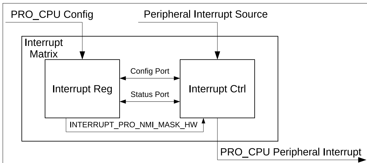
Figure 8.2-1. Interrupt Matrix Structure
