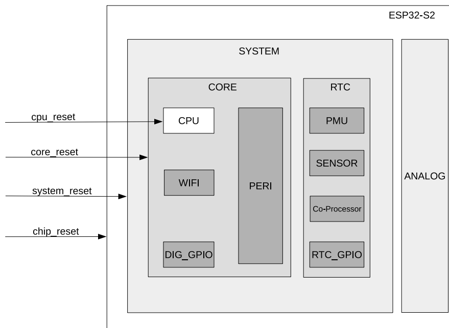
Figure 6.1-1. Reset Level
