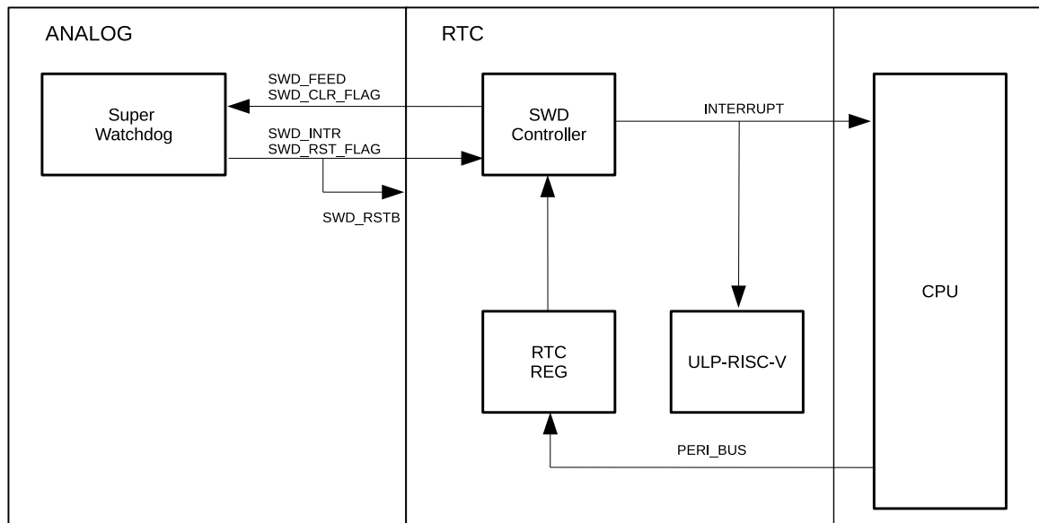
Figure 12.4-1. Super Watchdog Controller Structure
