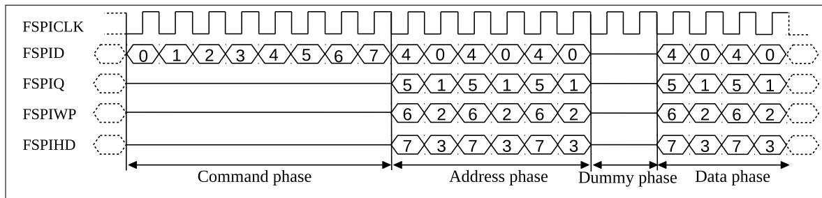
Figure 24.4-4. SPI Quad Read Command Sequence Sent by GP-SPI2 to Flash
