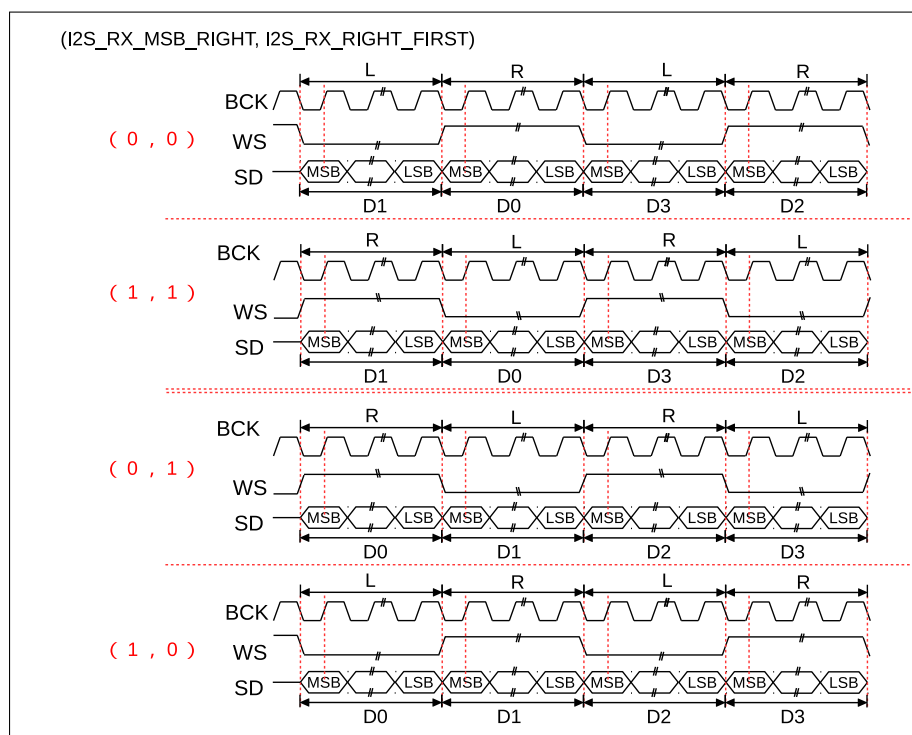
Figure 26.9-2. I2S RX Data When I2S_RX_DMA_EQUAL = 0
