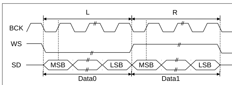
Figure 26.4-2. MSB Alignment Standard
