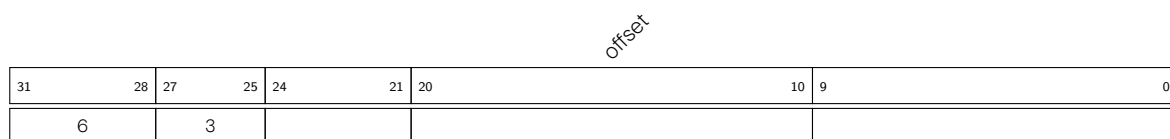
Figure 1.5-6. Instruction Type - Offset in Automatic Storage Mode (ST-OFFSET)
