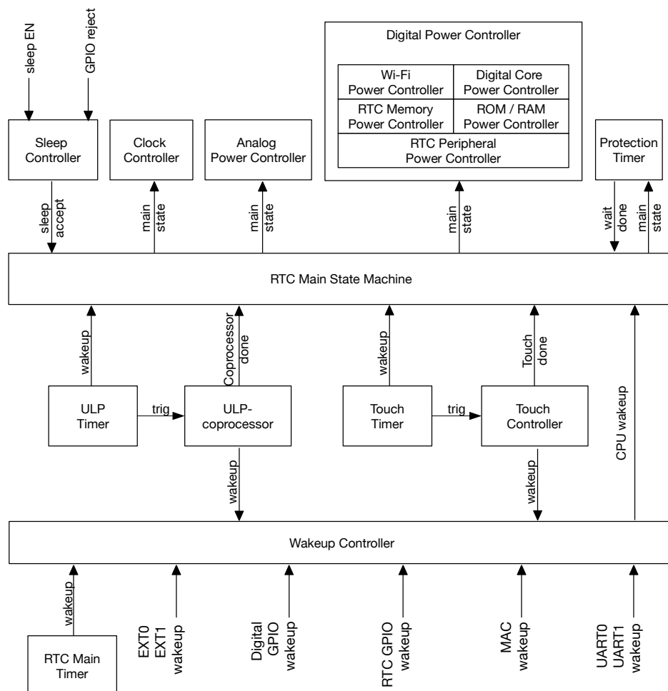
Figure 9.3-2. Power Management Unit Workflow
