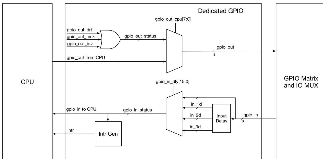
Figure 5.4-1. Dedicated GPIO Diagram
