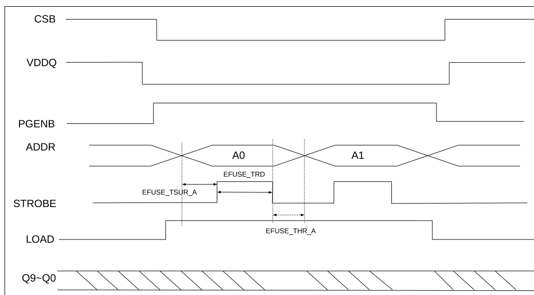
Figure 4.3-4. Timing Diagram for Reading eFuse
