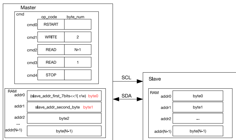
Figure 25.2-10. An I2C Master Reading an I2C Slave with a 10-bit Address
