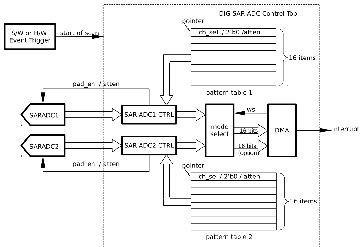
Figure 32.2-4. Diagram of DIG ADC Controllers
