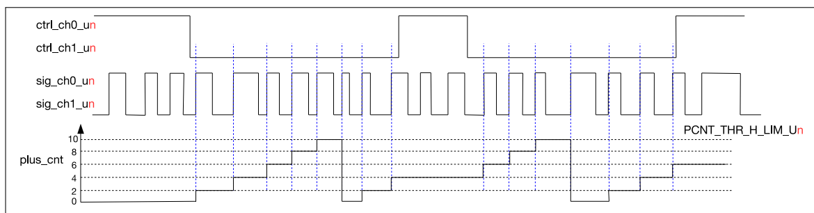
Figure 27.3-3. Two Channels Up Counting Diagram
