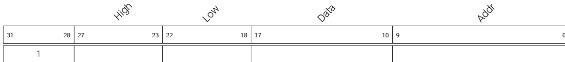
Figure 1.5-20. Instruction Type - REG_WR
