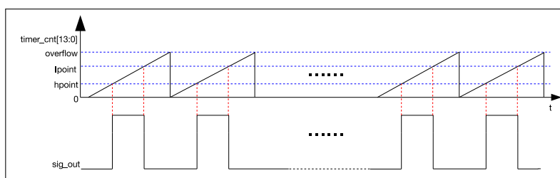
Figure 30.3-4. LED_PWM Output Signal Diagram
