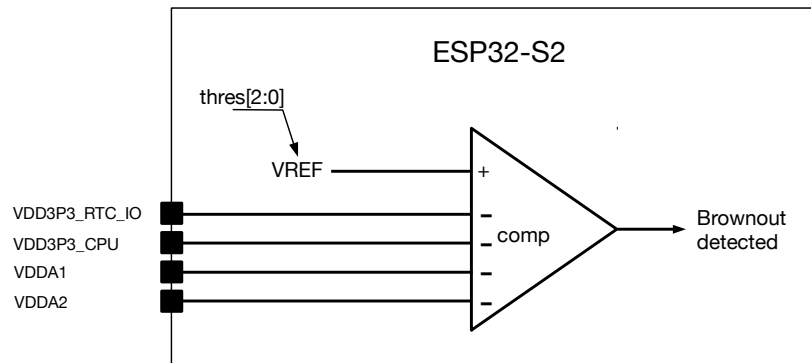
Figure 9.3-8. Brown-out detector
