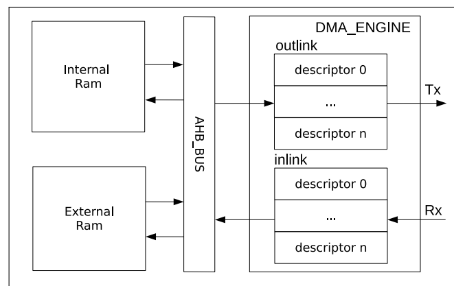
Figure 2.3-1. DMA Engine Architecture
