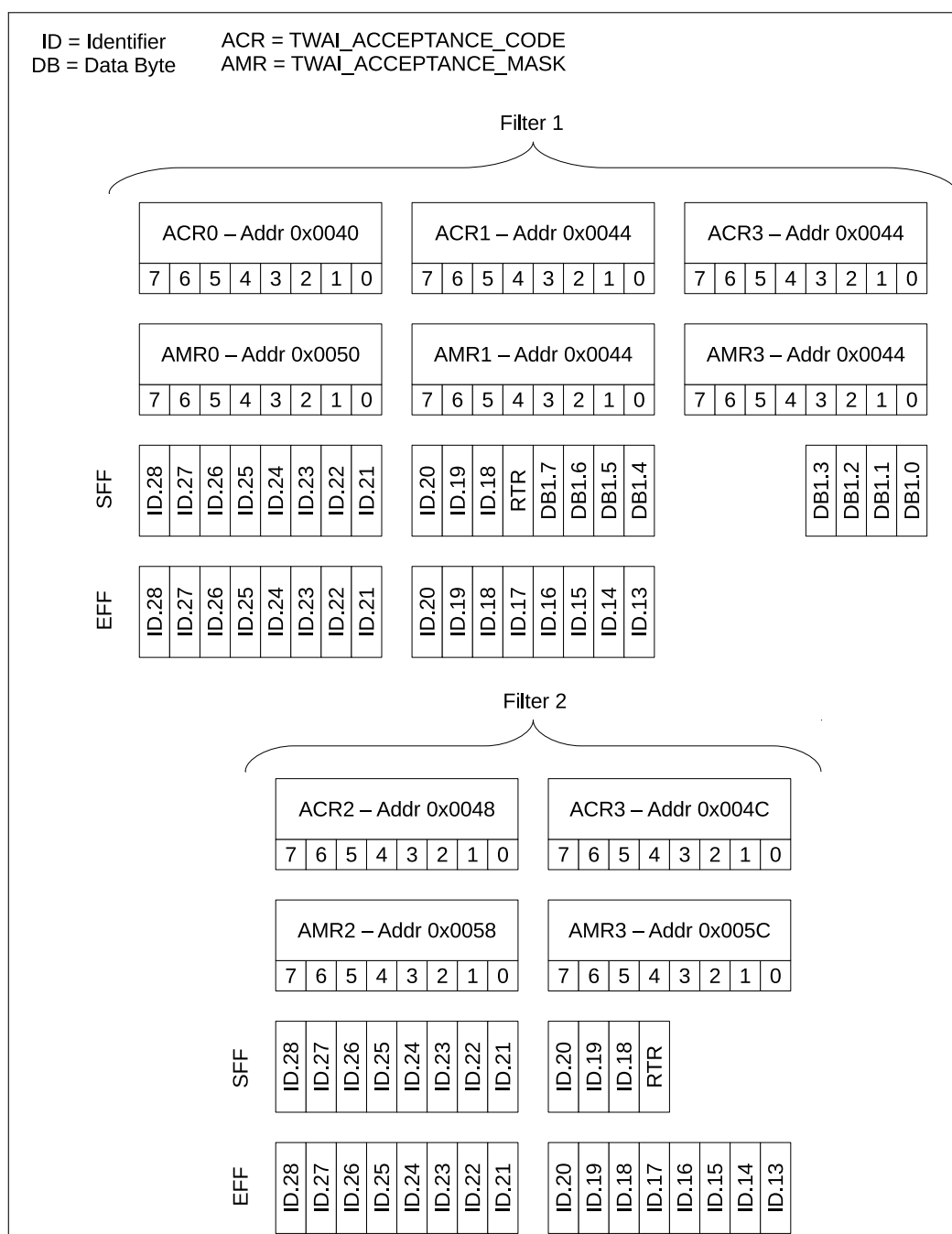
Figure 29.5-3. Dual Filter Mode
