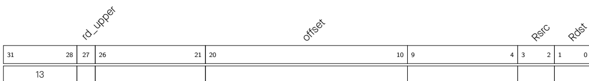
Figure 1.5-10. Instruction Type - LD
