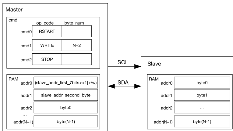
Figure 25.2-6. A Master Writing to a Slave with a 10-bit Address
