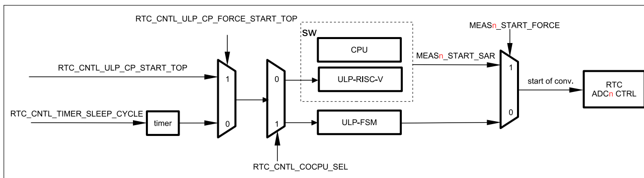
Figure 32.2-3. RTC SAR ADC Outline
