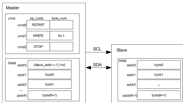
Figure 25.2-5. An I2C Master Writing to an I2C Slave with a 7-bit Address
