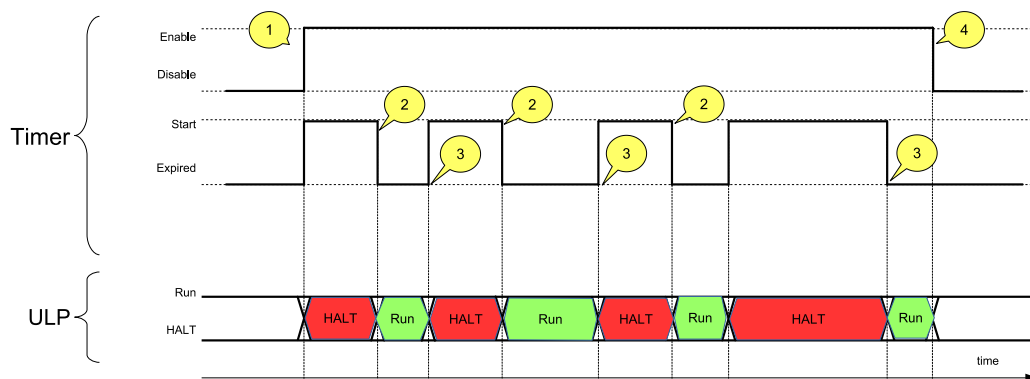
Figure 1.4-1. Sample of a ULP Operation Sequence
