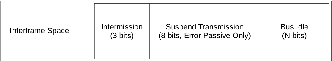
Figure 29.3-4. The Fields within an Interframe Space
