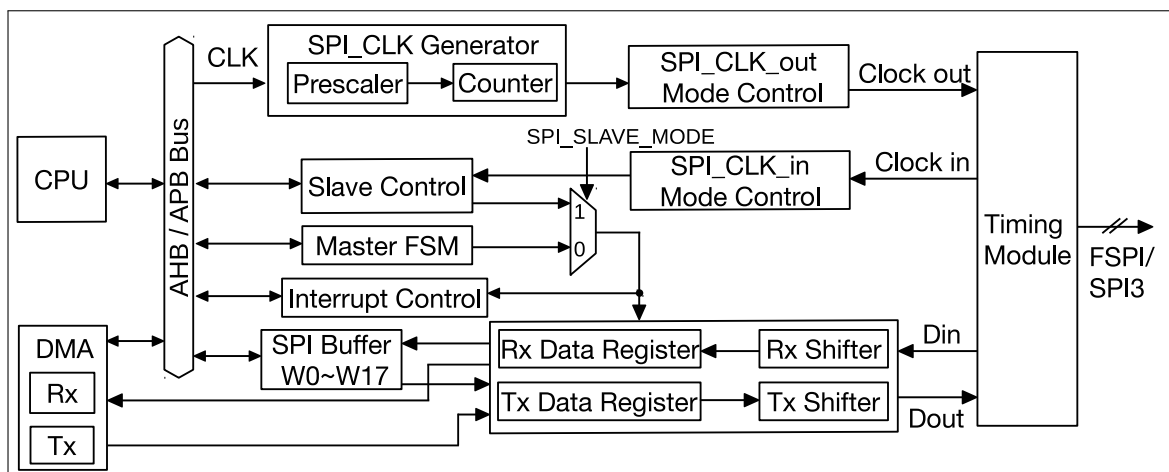
Figure 24.3-1. GP-SPI2/GP-SPI3 Block Diagram
