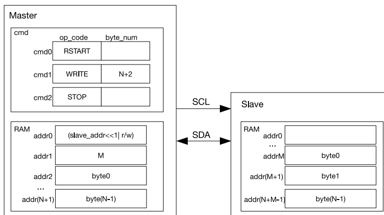
Figure 25.2-7. An I2C Master Writing Address M in the RAM to an I2C Slave with a 7-bit Address
