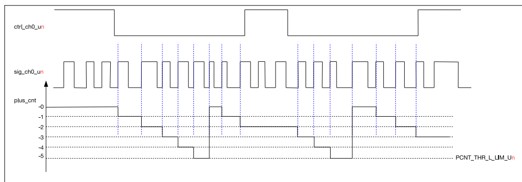
Figure 27.3-2. Channel 0 Down Counting Diagram
