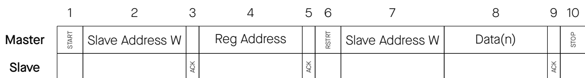
Figure 1.7-2. I2C Write Operation
