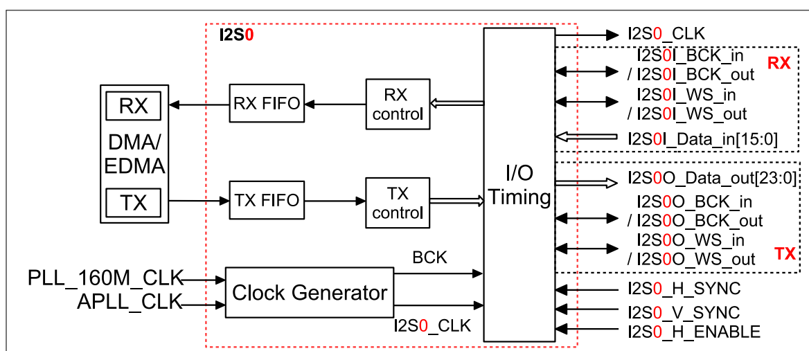
Figure 26.2-1. ESP32-S2 I2S System Diagram
