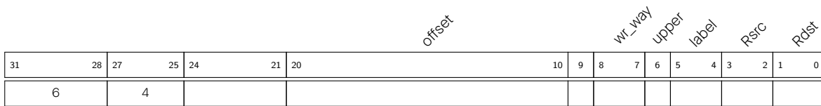
Figure 1.5-9. Instruction Type - Data Storage in Manual Storage Mode
