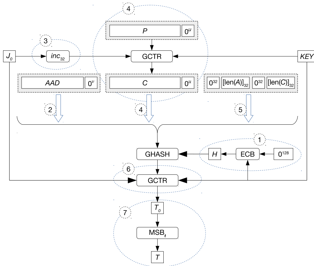
Figure 17.6-1. GCM Encryption Process
