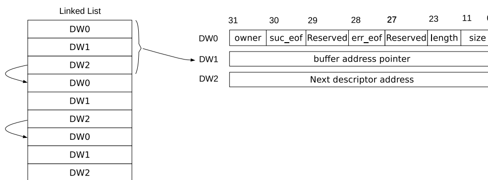
Figure 2.3-2. Structure of a Linked List
