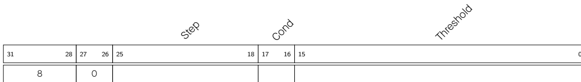
Figure 1.5-12. Instruction Type - JUMPR
