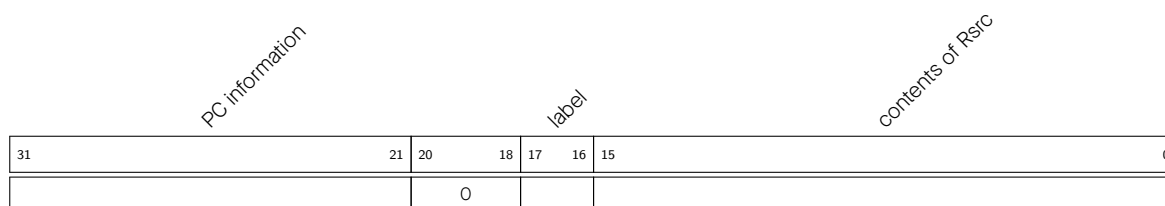
Figure 1.5-8. Data Structure of RTC_SLOW_MEM[Rdst + Offset]
