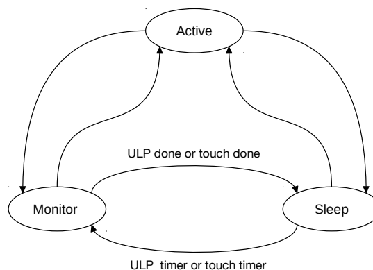
Figure 9.4-1. RTC States Transition
