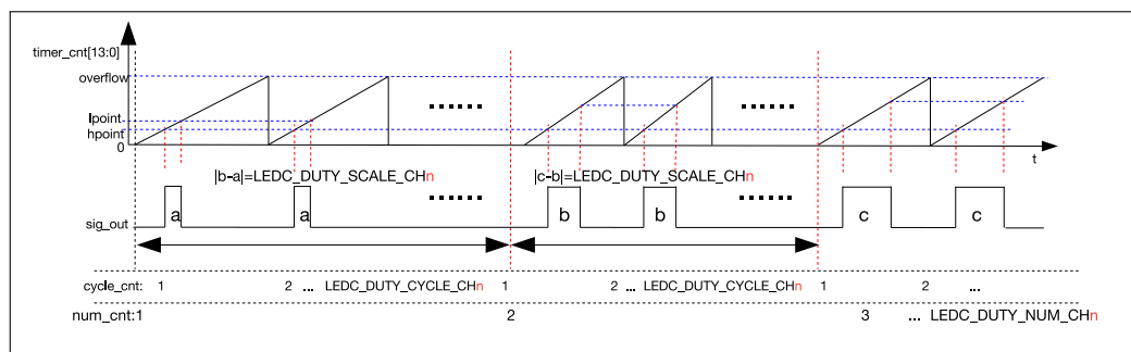
Figure 30.3-5. Output Signal Diagram of Fading Duty Cycle
