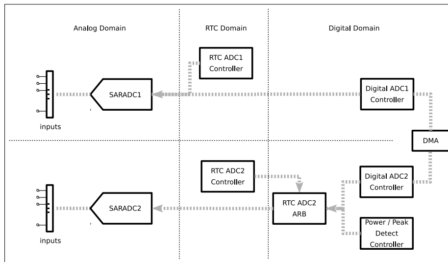
Figure 32.2-1. SAR ADC Overview
