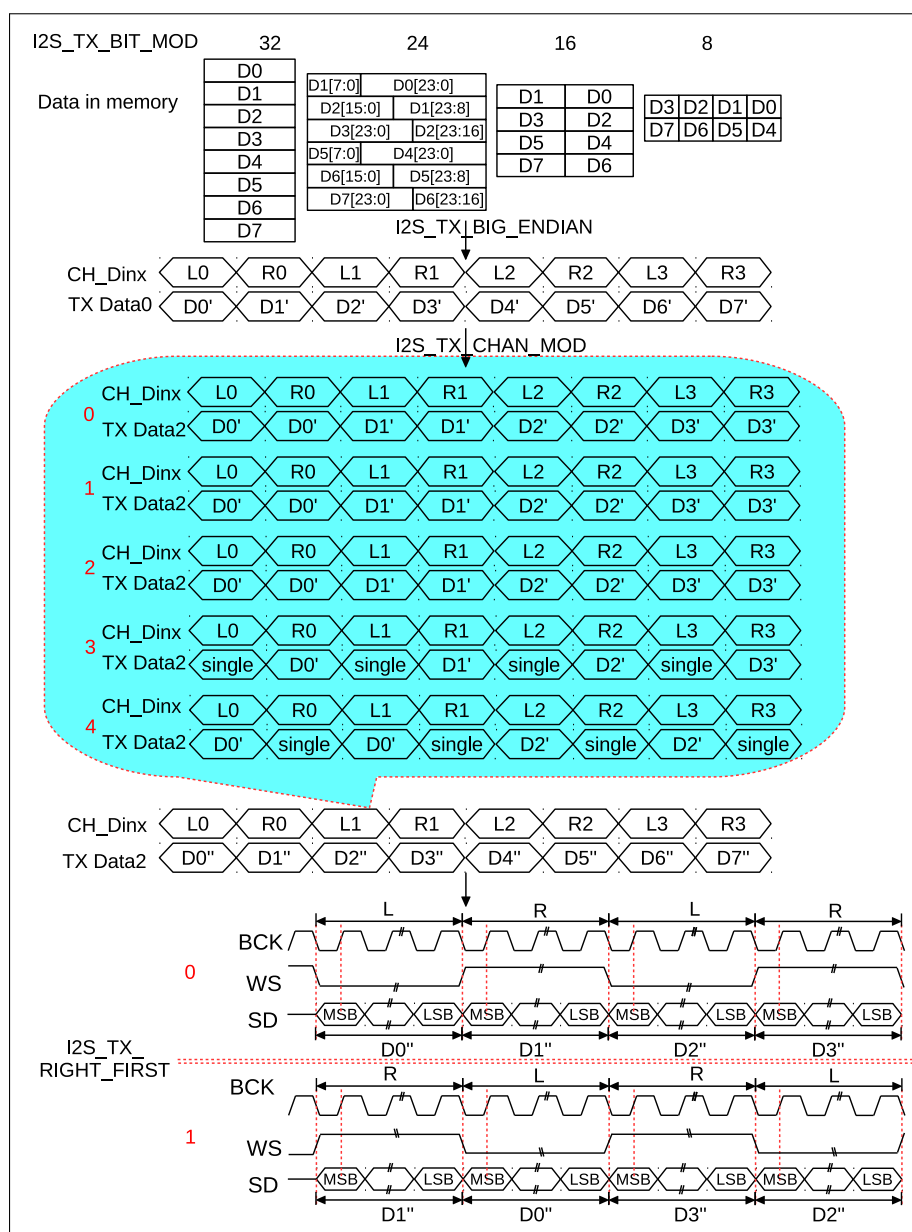
Figure 26.8-3. I2S TX Data When I2S_TX_DMA_EQUAL = 1
