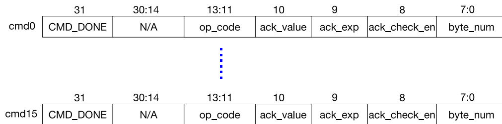
Figure 25.2-3. Structure of I2C Command Register
