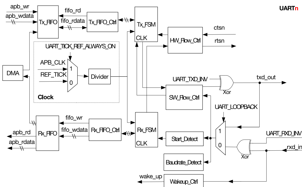
Figure 23.3-1. UART Structure
