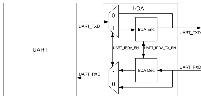
Figure 23.3-9. IrDA Encoding and Decoding Diagram
