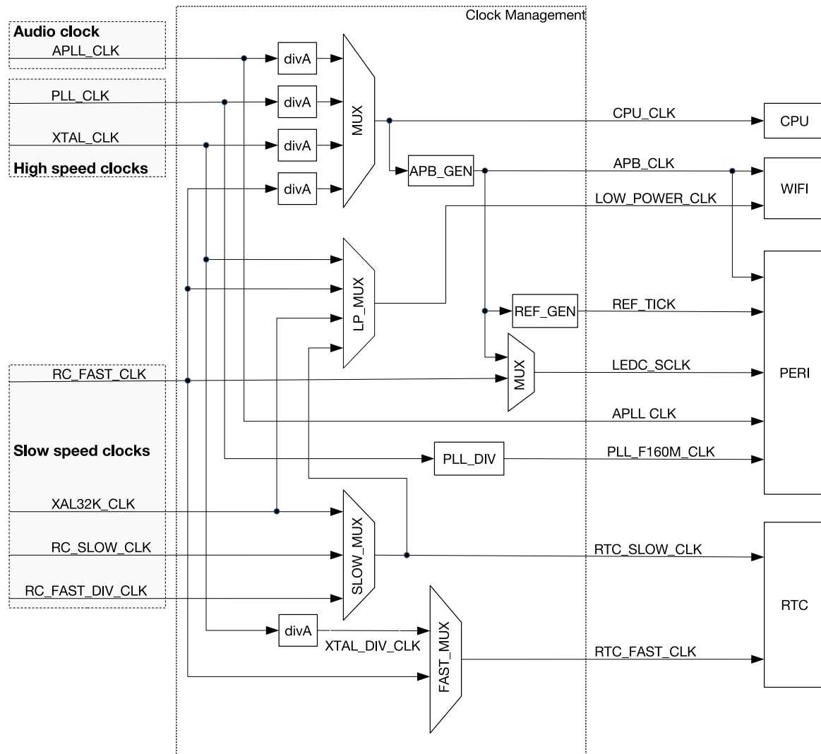
Figure 6.2-1. System Clock
