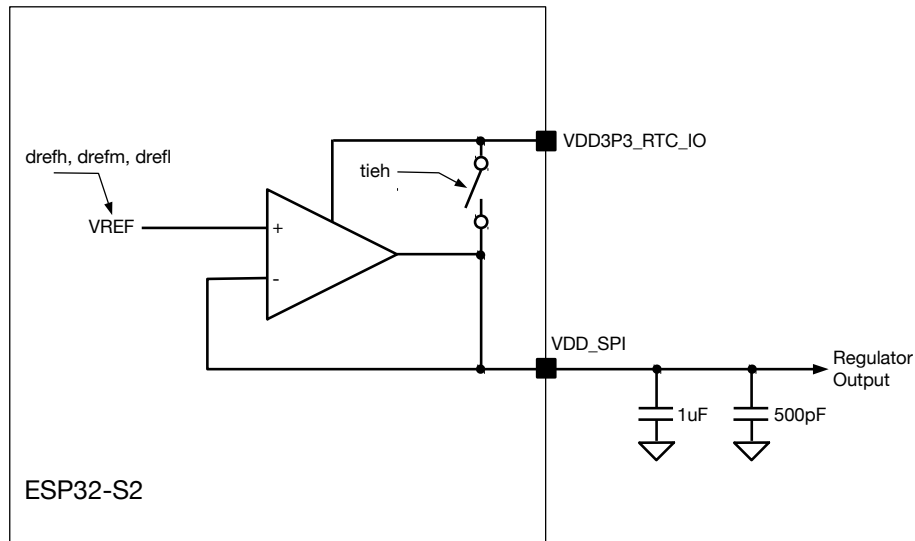
Figure 9.3-7. Flash voltage regulator
