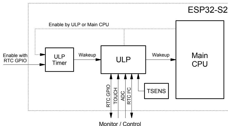
Figure 1.1-1. ULP Coprocessor Overview
