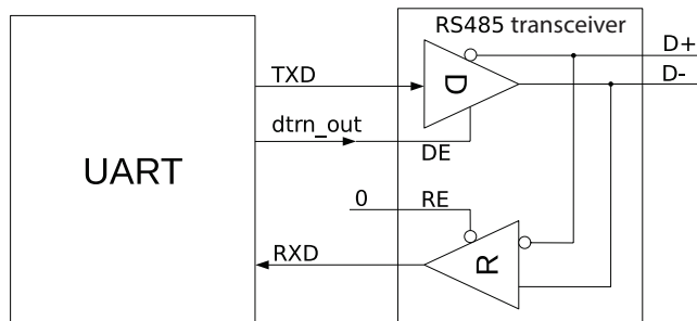
Figure 23.3-7. Driver Control Diagram in RS485 Mode
