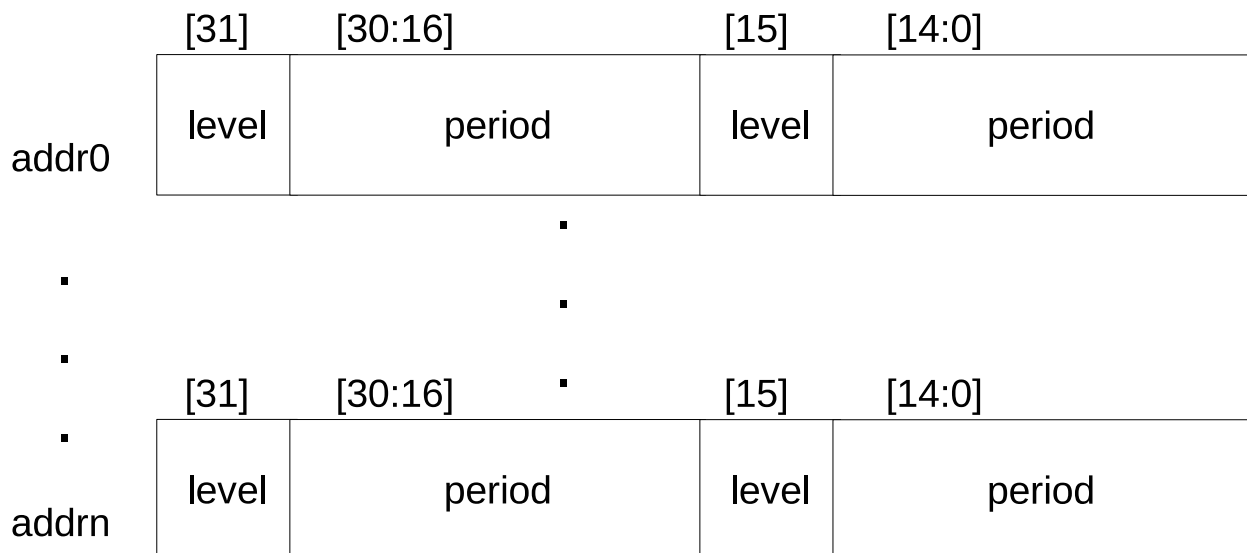
Figure 31.2-3. Format of Pulse Code in RAM
