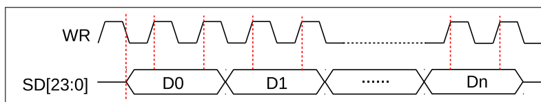
Figure 26.10-3. Data Frame Format 2 in LCD Master Transmitting Mode
