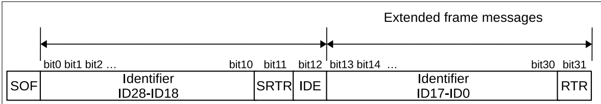
Figure 29.5-5. Positions of Arbitration Lost Bits
