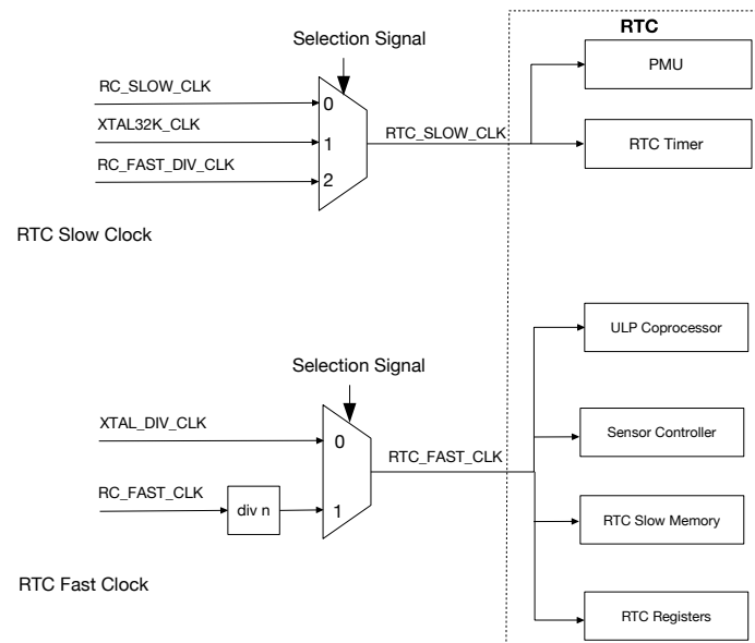
Figure 9.3-3. RTC_FAST_CLK and RTC_SLOW_CLK
