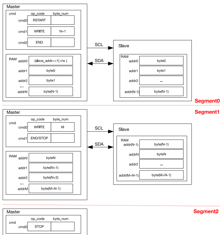
Figure 25.2-8. An I2C Master Writing to an I2C Slave with a 7-bit Address in Multiple Sequences
