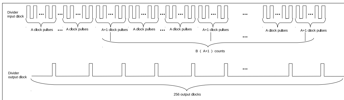
Figure 30.3-3. LED_PWM Divider
