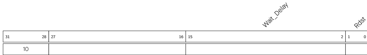
Figure 1.5-17. Instruction Type - TSENS
