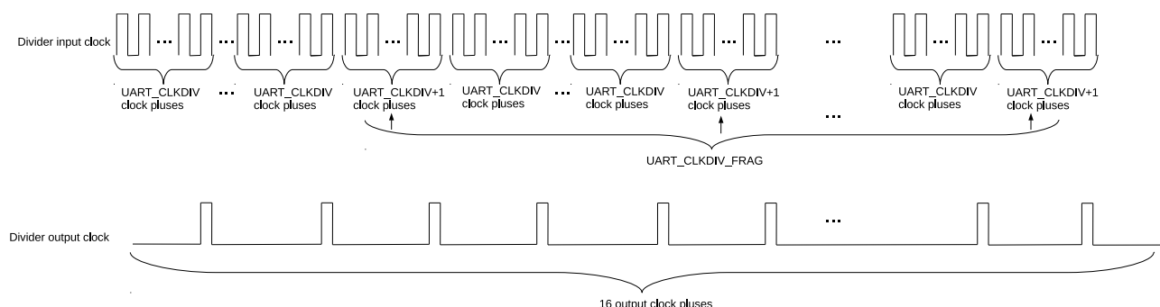
Figure 23.3-3. UART Controllers Division
