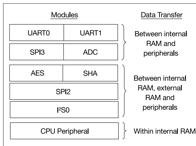
Figure 2.1-1. Modules with DMA and Supported Data Transfers
