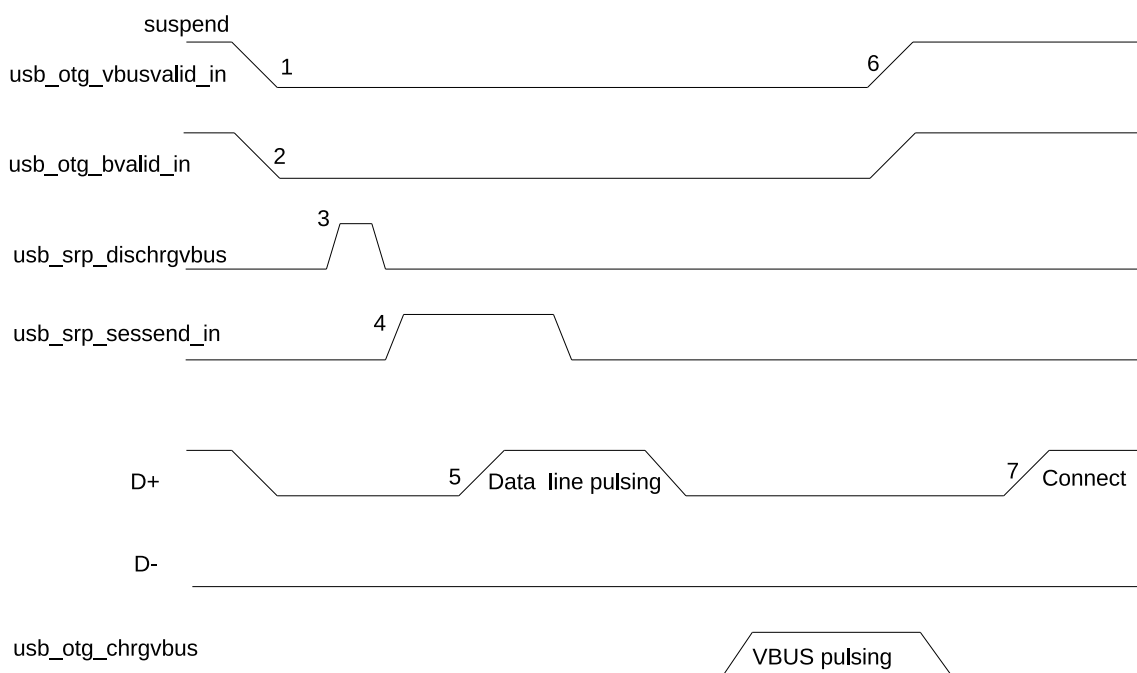
Figure 28.4-2. B-Device SRP
