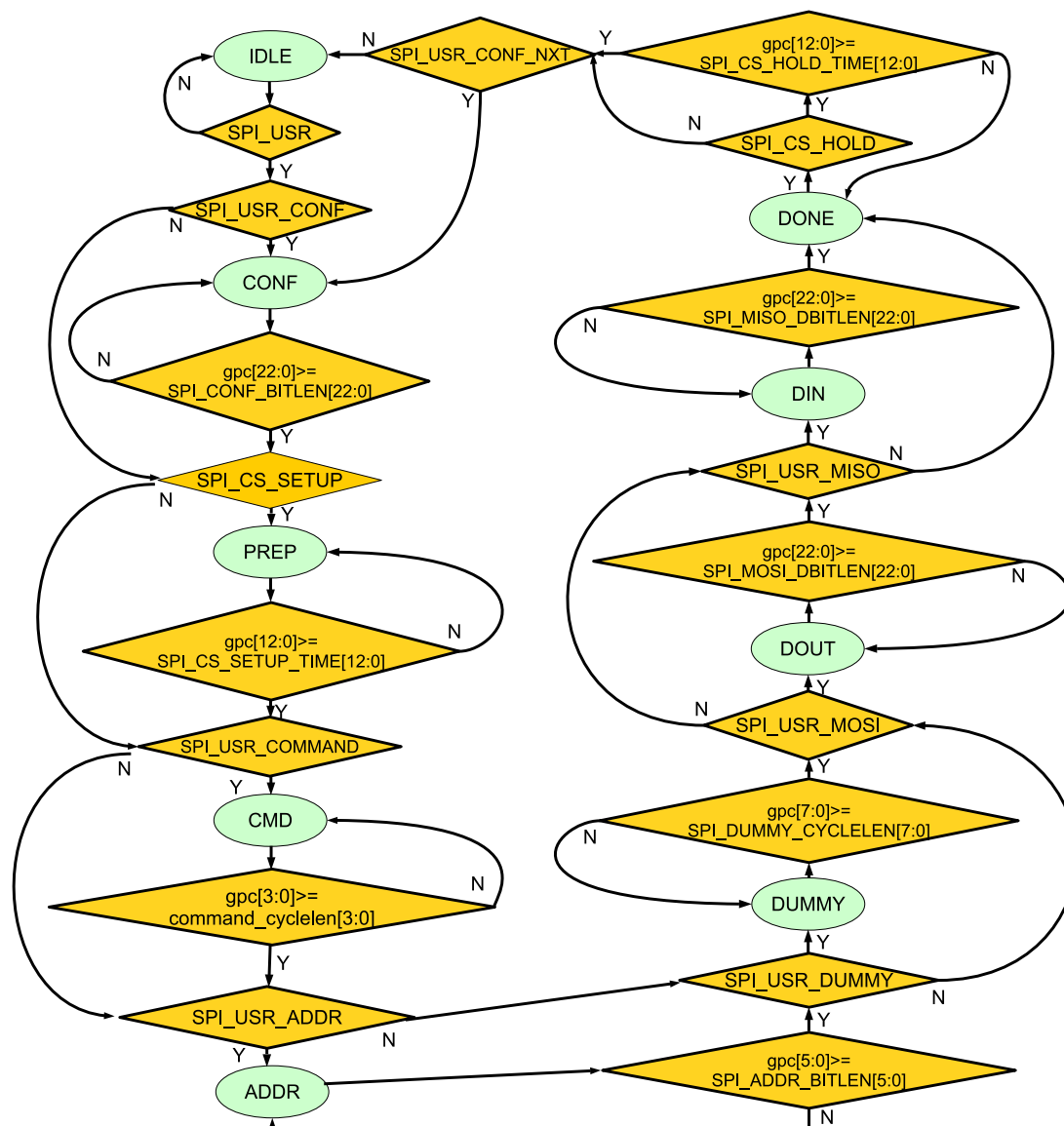
Figure 24.4-1. GP-SPI2 State Flow in Master Mode
