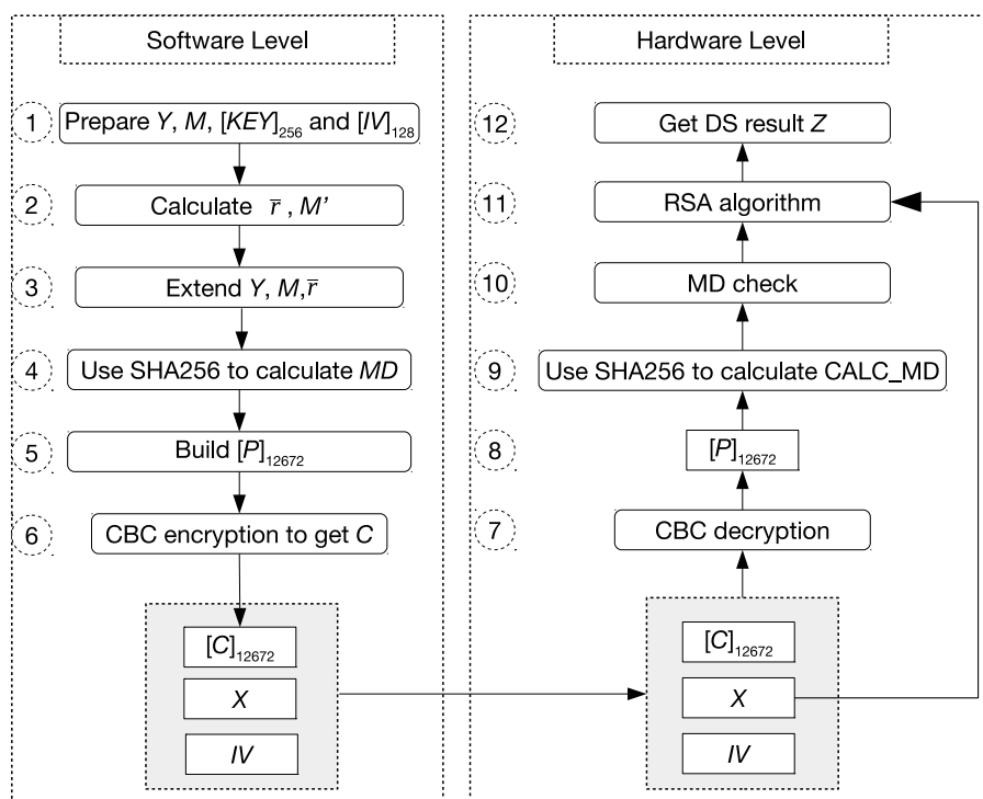
Figure 20.3-1. Preparations and DS Operation
