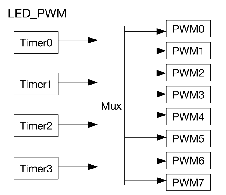
Figure 30.3-1. LED_PWM Architecture
