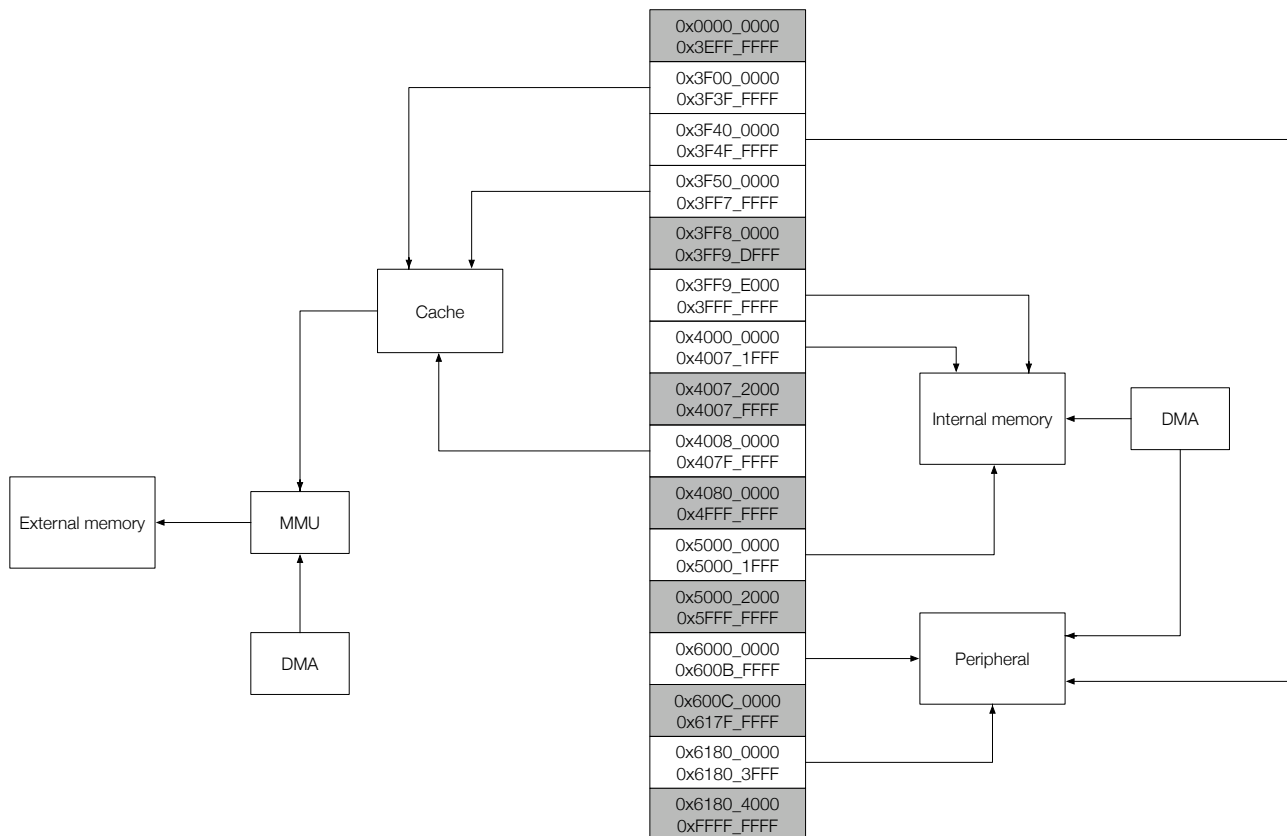
Figure 3.2-1. System Structure and Address Mapping
