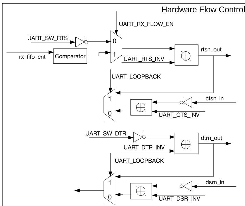
Figure 23.3-10. Hardware Flow Control Diagram
