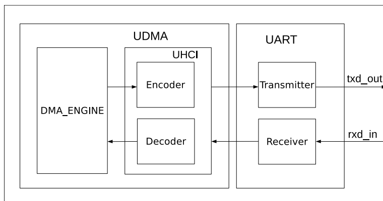
Figure 2.5-1. Data Transfer in UDMA Mode
