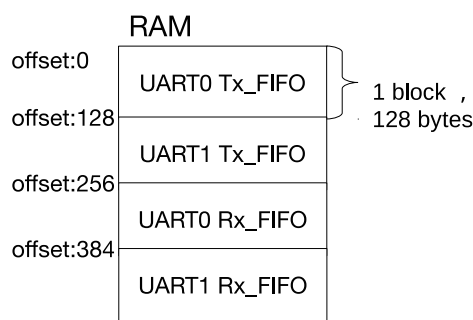
Figure 23.3-2. UART Controllers Sharing RAM
