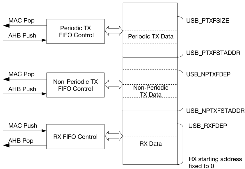
Figure 28.3-3. Host Mode FIFOs
