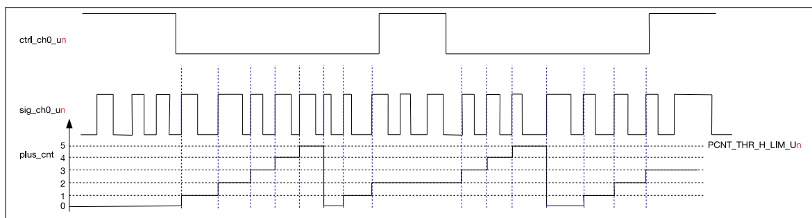
Figure 27.3-1. Channel 0 Up Counting Diagram
