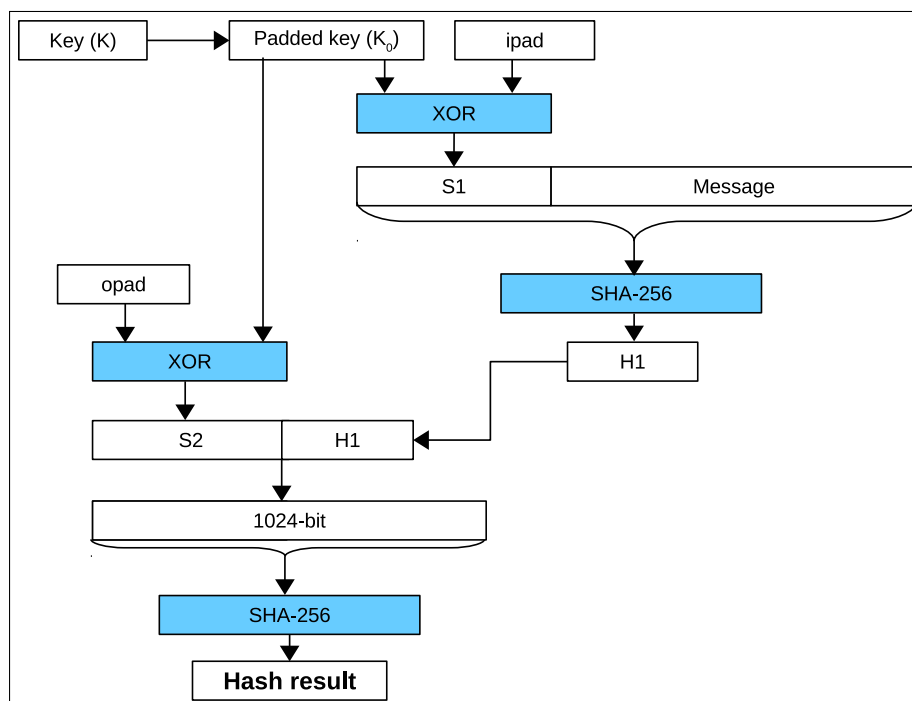
Figure 19.4-2. HMAC Structure Schematic Diagram
