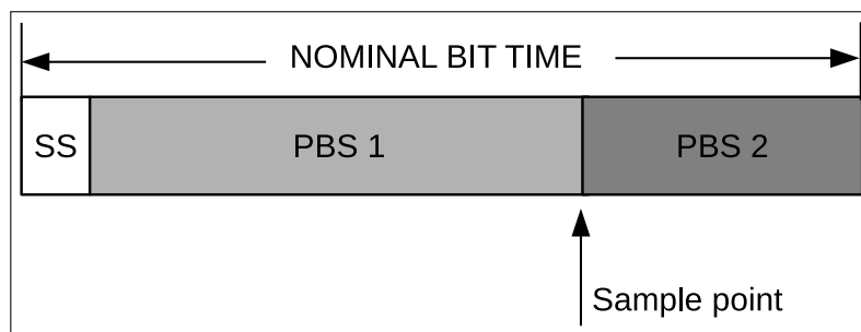
Figure 29.3-5. Layout of a Bit
