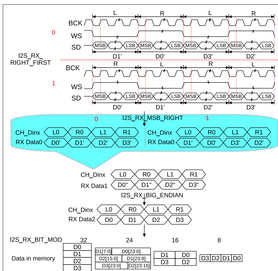
Figure 26.9-1. I2S RX Data When I2S_RX_DMA_EQUAL = 0
