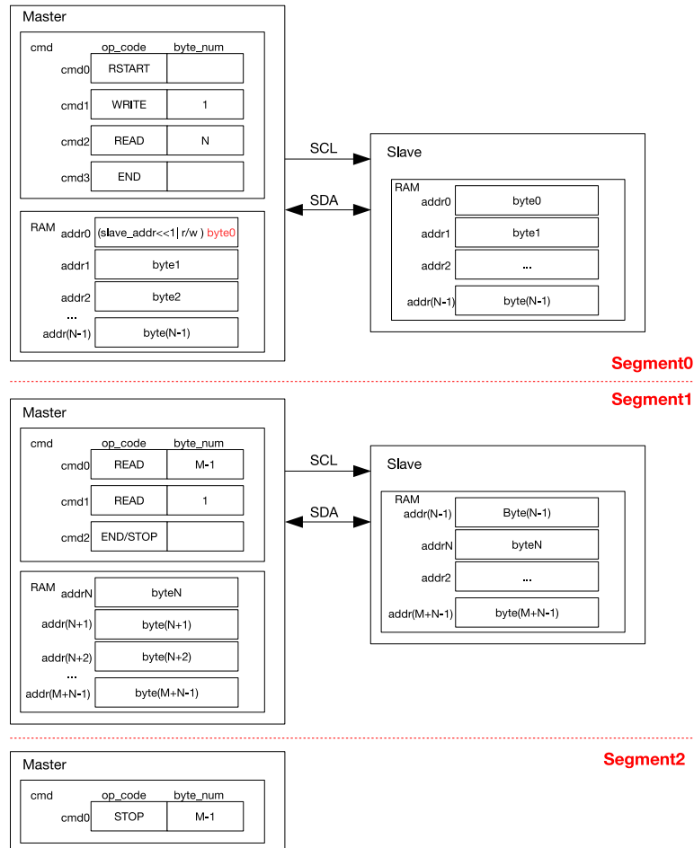
Figure 25.2-12. An I2C Master Reading an I2C Slave with a 7-bit Address in Segments
