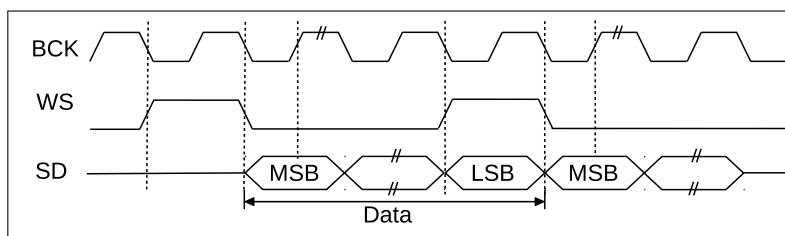
Figure 26.4-3. PCM Standard
