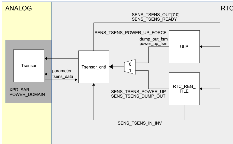
Figure 32.4-1. Structure of Temperature Sensor
