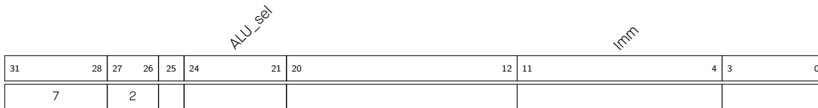
Figure 1.5-4. Instruction Type — ALU for Operations with Stage Count Register
