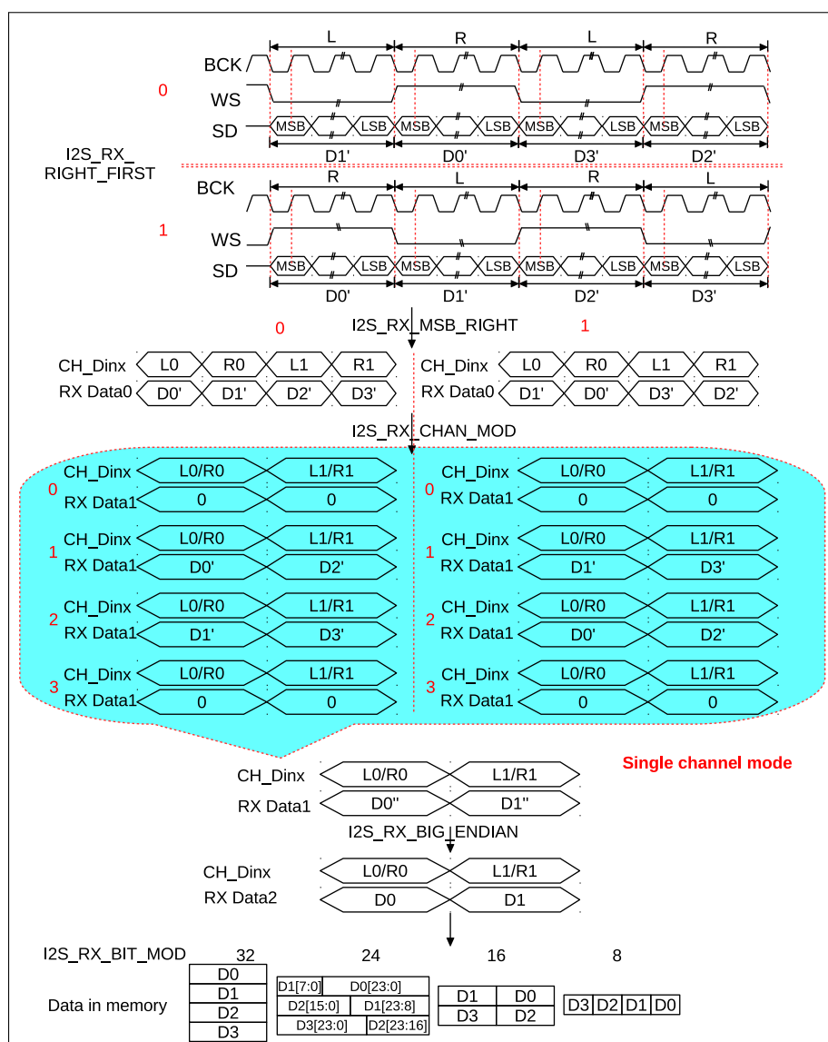
Figure 26.9-3. ESP32-S2 I2S RX Data When I2S_RX_DMA_EQUAL = 1
