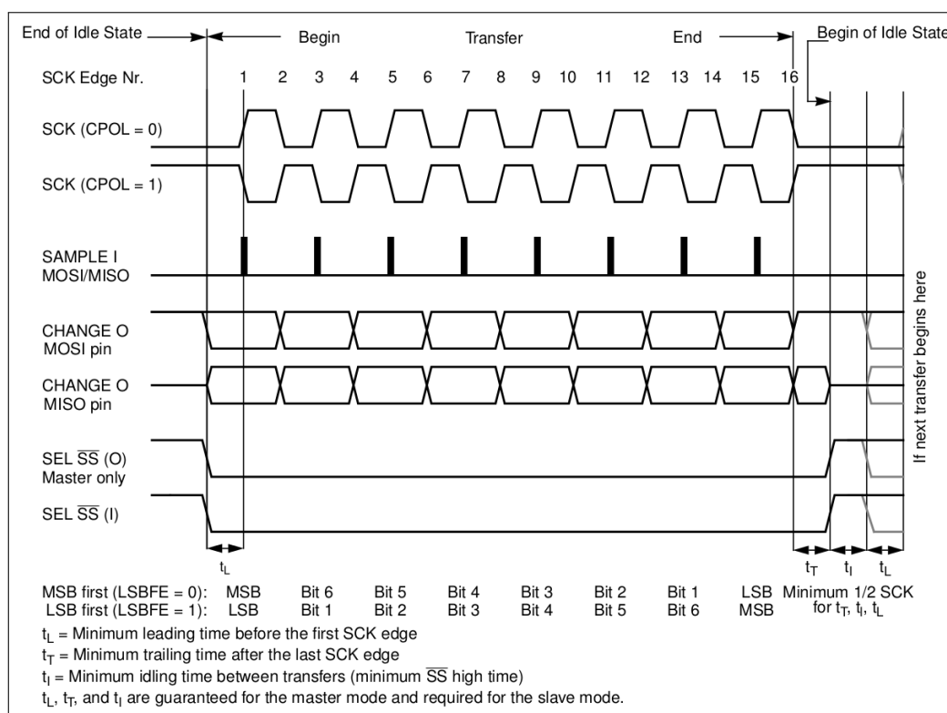
Figure 24.9-1. SPI CLK Mode 0 or 2
