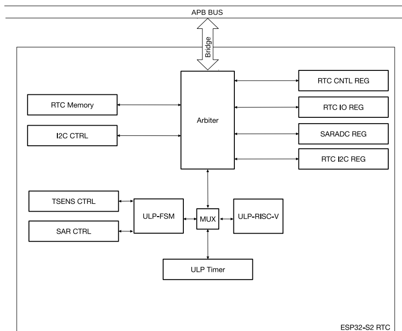
Figure 1.2-1. ULP Coprocessor Diagram
