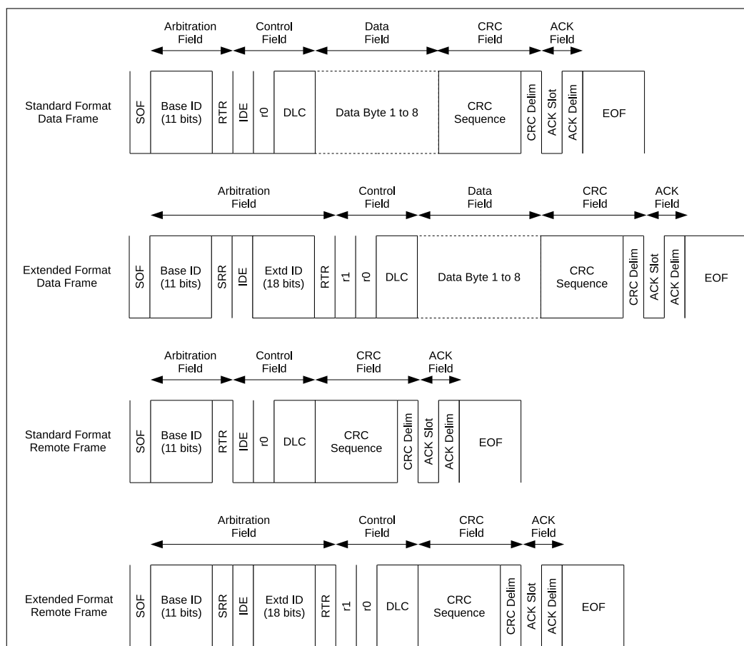
Figure 29.3-1. The bit fields of Data Frames and Remote Frames
