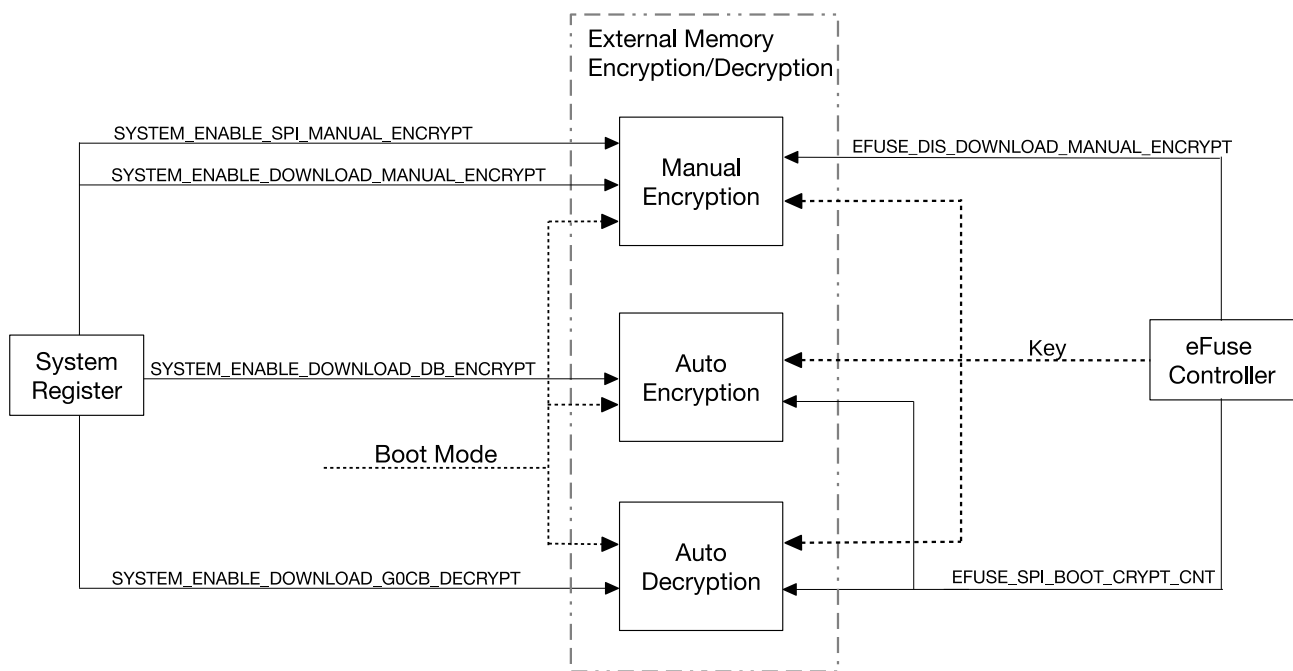
Figure 21.3-1. Architecture of the External Memory Encryption and Decryption Module
