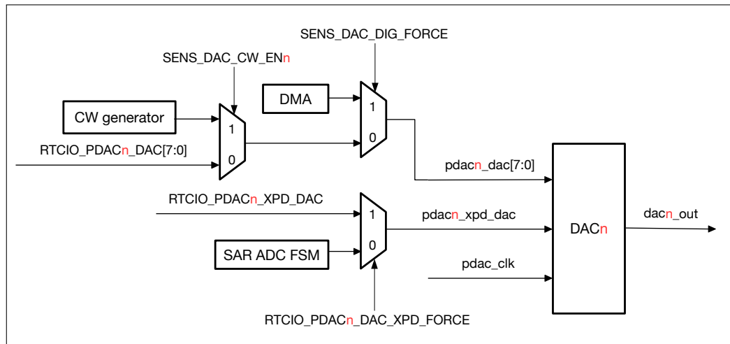
Figure 32.3-1. Diagram of DAC Function
