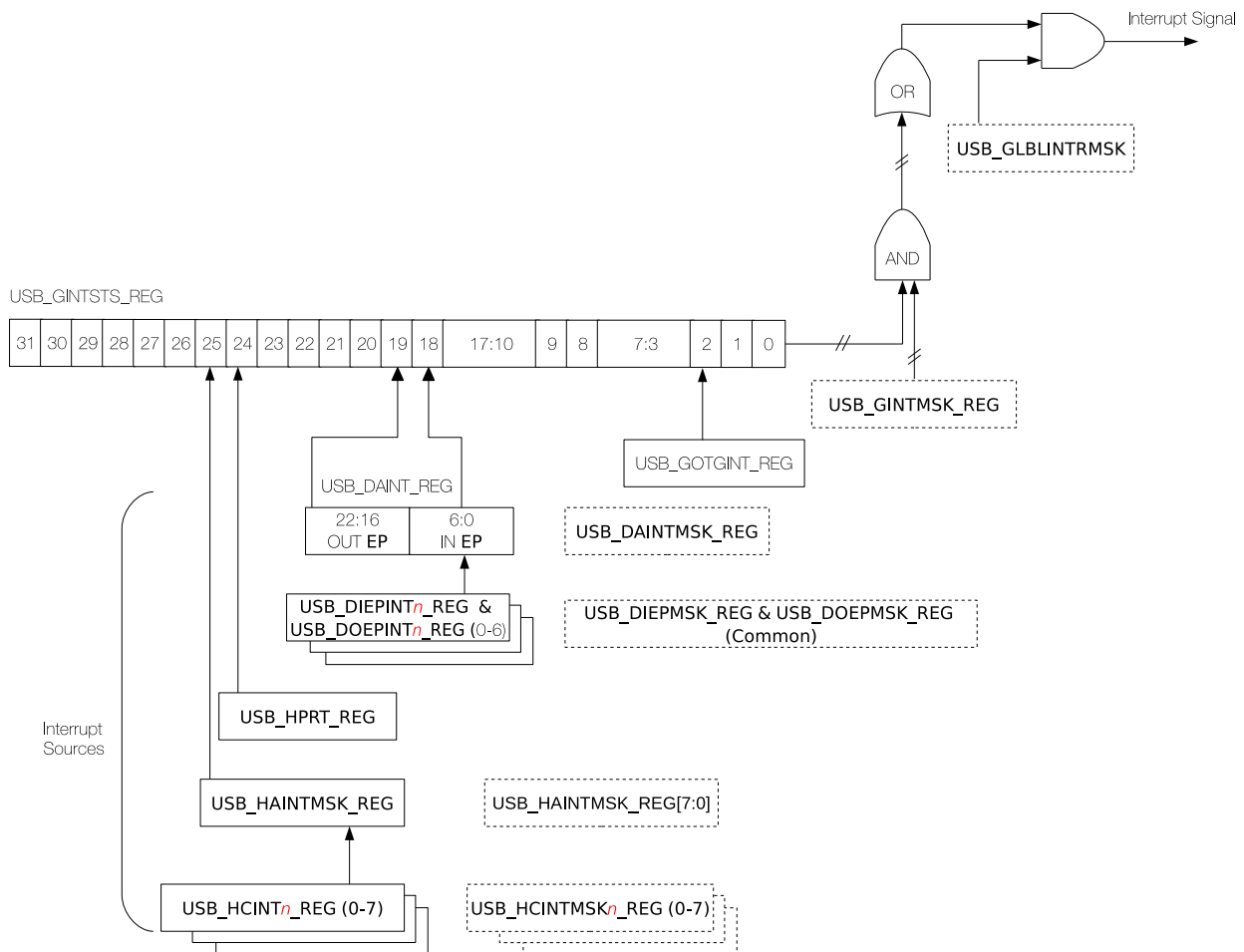
Figure 28.3-5. OTG_FS Interrupt Hierarchy
