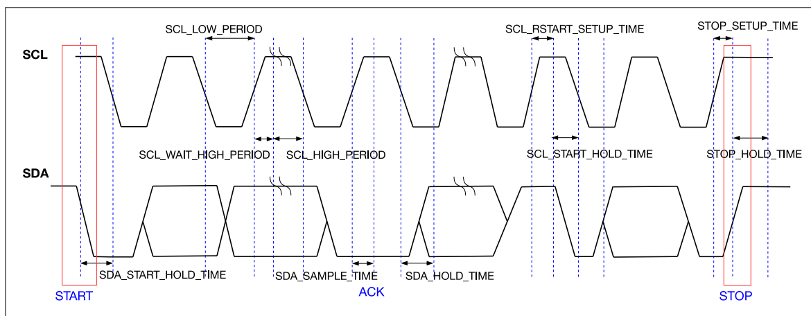
Figure 25.2-4. I2C Timing Diagram
