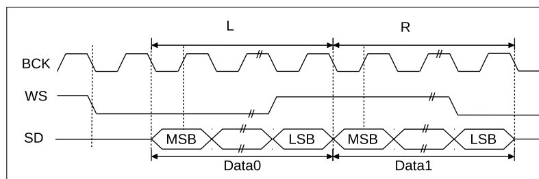
Figure 26.4-1. Philips Standard
