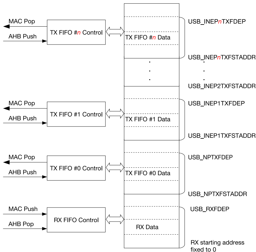
Figure 28.3-4. Device Mode FIFOs
