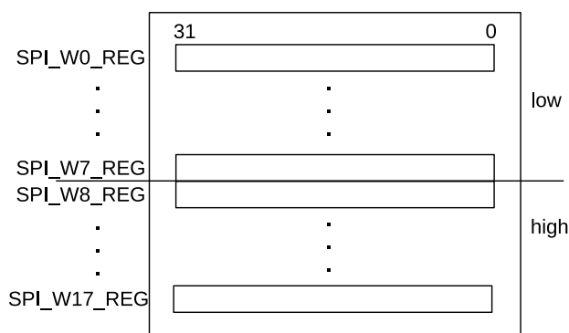
Figure 24.7-1. Data Buffer Used in CPU-Controlled Mode
