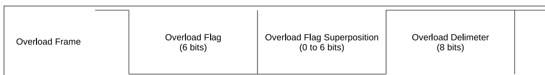
Figure 29.3-3. The Bit Fields of an Overload Frame
