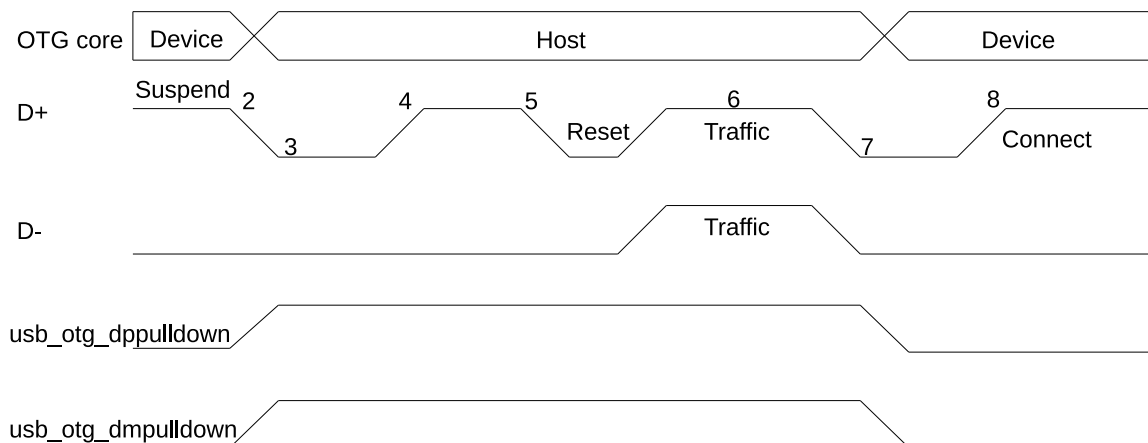
Figure 28.4-4. B-Device HNP
