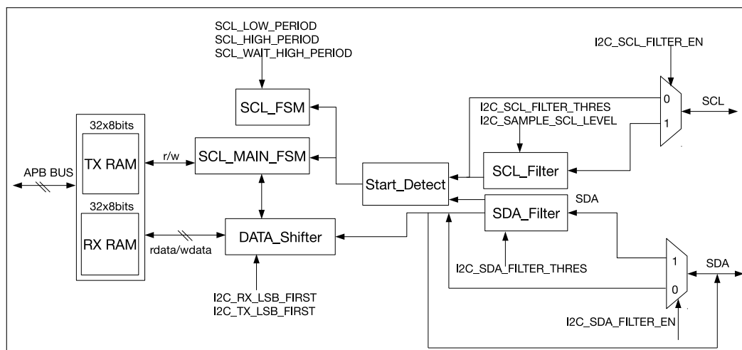
Figure 25.2-2. I2C Slave Architecture
