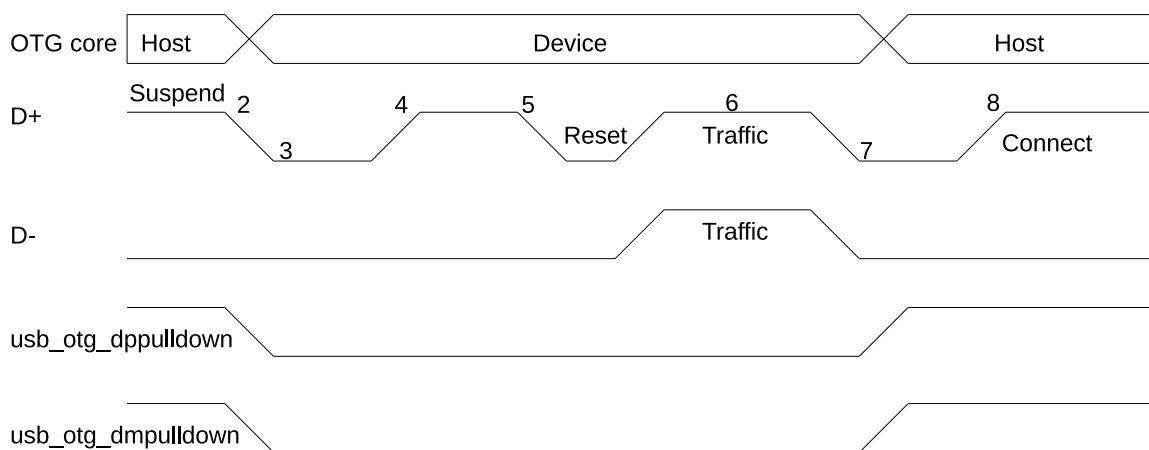
Figure 28.4-3. A-Device HNP
