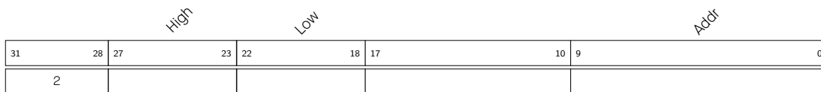
Figure 1.5-19. Instruction Type - REG_RD
