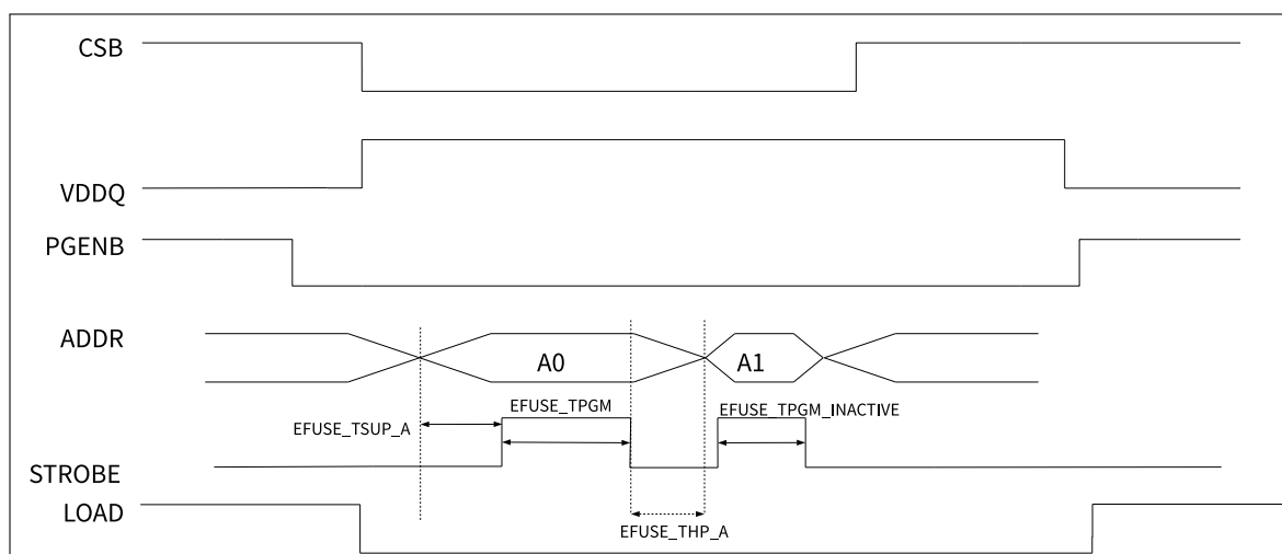
Figure 4.3-3. eFuse-Programming Timing Diagram
