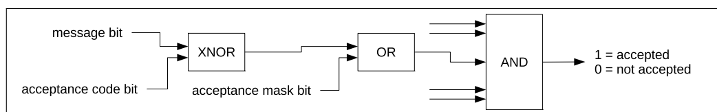
Figure 29.5-1. Acceptance Filter
