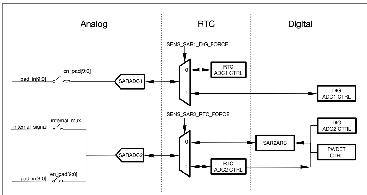
Figure 32.2-2. SAR ADC Function Overview
