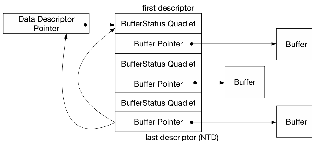
Figure 28.3-6. Scatter/Gather DMA Descriptor List
