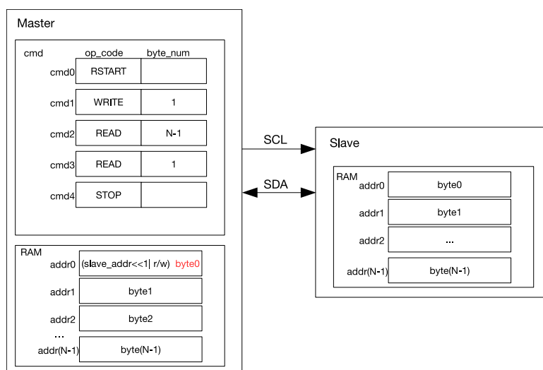
Figure 25.2-9. An I2C Master Reading an I2C Slave with a 7-bit Address
