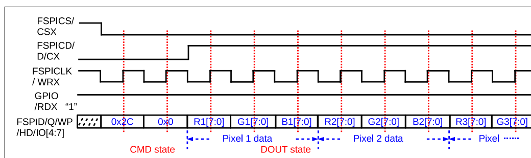
Figure 24.4-6. Write Command Sequence to an 8-bit LCD Driver
