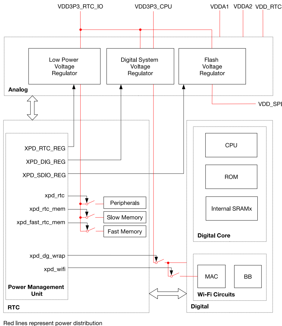
Figure 9.3-1. Low-power Management Schematics
