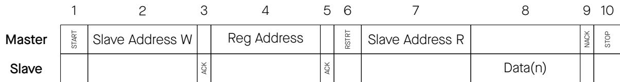
Figure 1.7-1. I2C Read Operation
