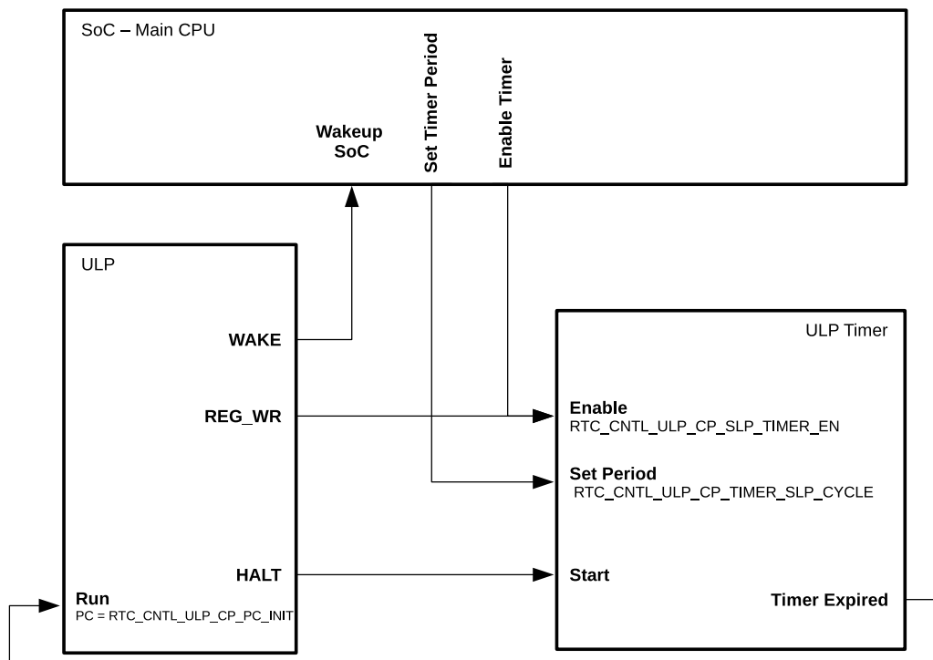
Figure 1.4-2. Control of ULP Program Execution
