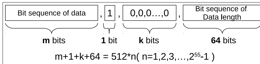
Figure 19.4-1. HMAC SHA-256 Padding Diagram
