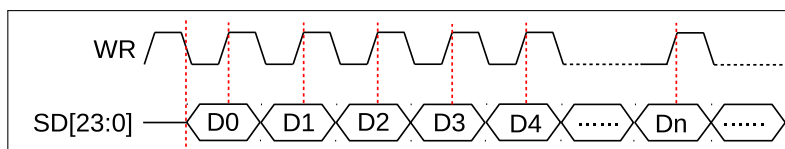
Figure 26.10-2. Data Frame Format 1 in LCD Master Transmitting Mode
