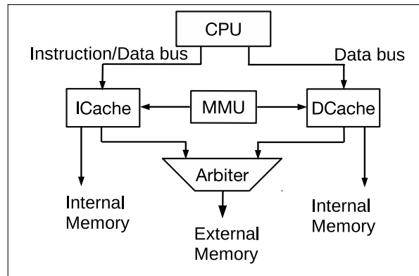
Figure 3.3-1. Cache Structure
