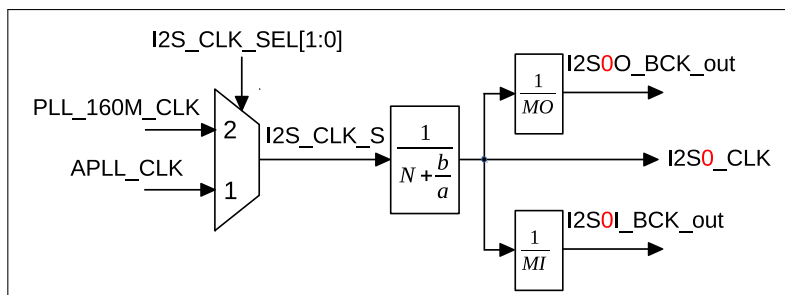
Figure 26.5-1. I2S Clock
