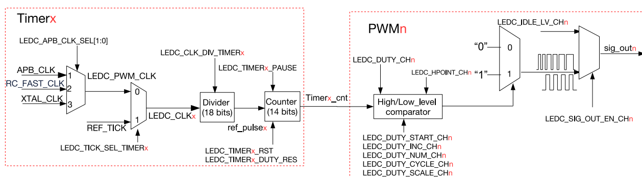
Figure 30.3-2. LED_PWM generator Diagram
