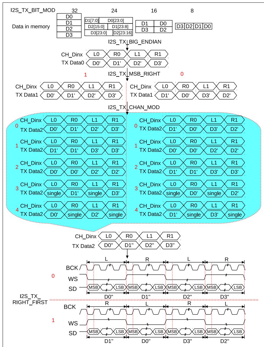
Figure 26.8-1. ESP32-S2 I2S Data Transmitting Flow When I2S_TX_DMA_EQUAL = 0
