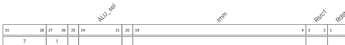
Figure 1.5-3. Instruction Type — ALU for Operations with Immediate Value
