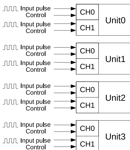
Figure 27.0-1. PCNT Block Diagram
