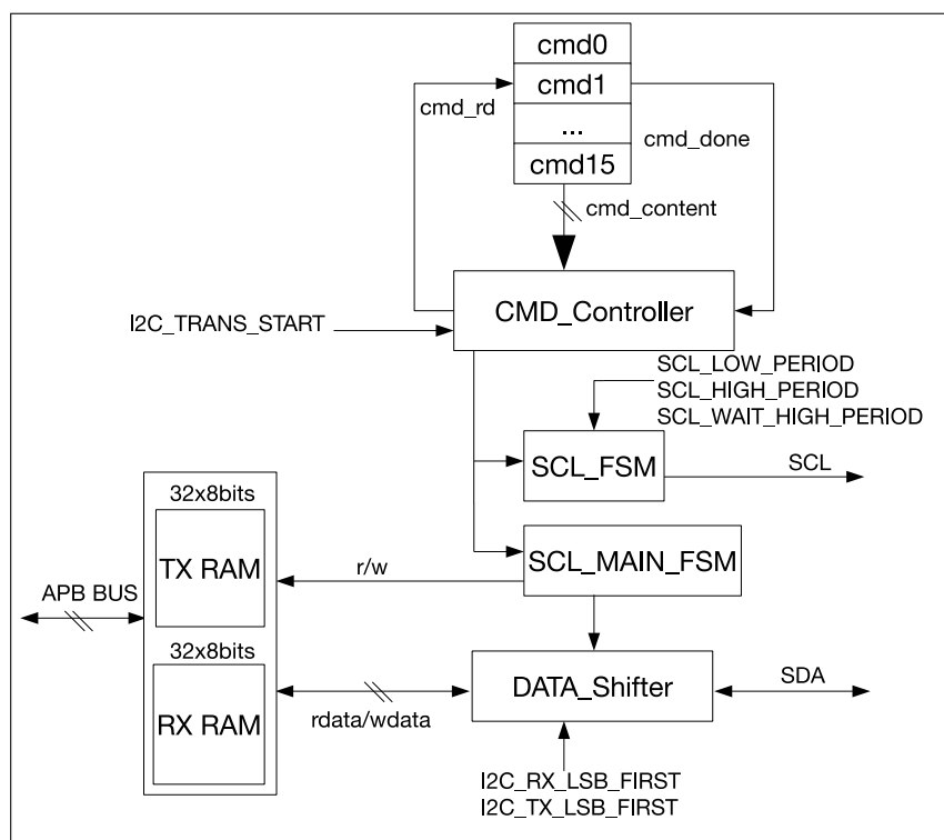
Figure 25.2-1. I2C Master Architecture
